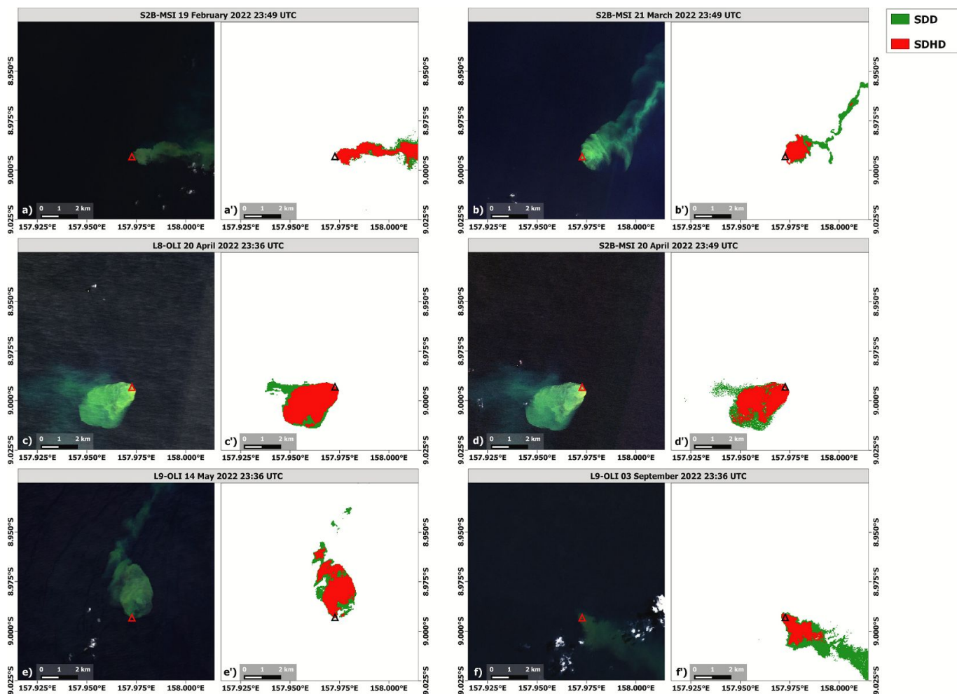
Fig. 5. Discoloration maps by the SDD/SDHD algorithms. S2A/B-MSI and L8/9-OLI imagery in true color composite (Red, Green, Blue2) for the selected test dates (a, b, c, d, e, f). Discoloration maps derived by the SDD (green) and SDHD (red) algorithms for the corresponding test dates (a', b', c', d', e', f). The white pixels on the discoloration maps represent the discarded ones, namely cloudy/no data or other water pixels. The location of Kavachi is shown by the red and black triangles in the (a–f) and (a'–f') panels, respectively. (For interpretation of the references to color in this figure legend, the reader is referred to the web version of this article.)
