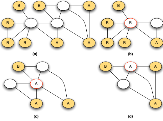
Fig. 4: Ego-network based quantification. (a) the full graph with labeled and unlabeled nodes; (b-c-d) 1-hop ego-networks of the unlabeled nodes.
