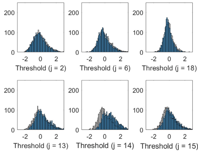
Fig. 9. Statistical distribution of the normalized Cornwell index (FF BCs, case A2 (Section 5), \sigma_j^{(i)} = 0.005 ). The distribution relative to damage case is represented in a darker color. (For interpretation of the references to color in this figure legend, the reader is referred to the web version of this article.)
