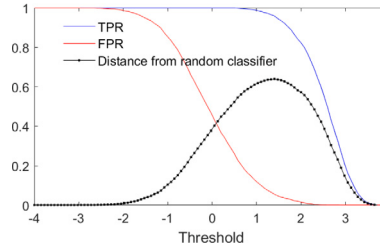
Fig. 13. TPR, FPR and Distance from random classifier of the Cornwell index ( \sigma_j^{(i)} = 0.001 , FF BCs, damage case A2).
