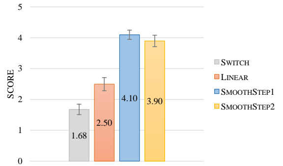
Figure 9: Subjective evaluation. Average scores and 95% confidence intervals of the four tested techniques without the subjects detected as outliers. Note the high preference of the methods SMOOTHSTEP1 and SMOOTHSTEP2 w.r.t to the other techniques.
