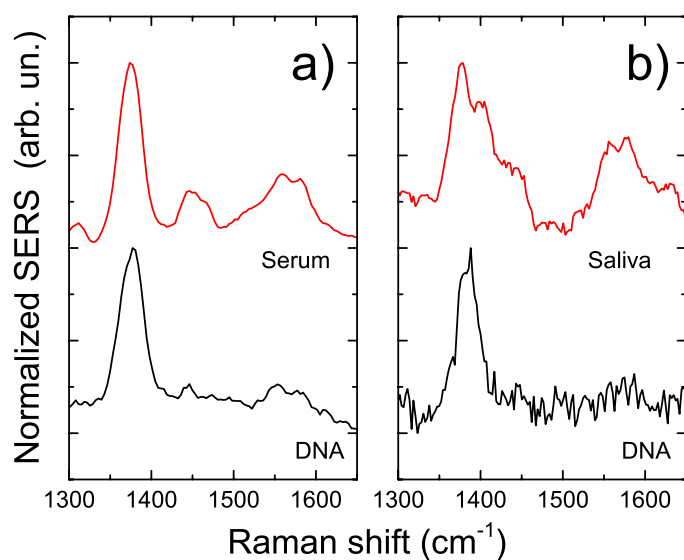
Figure 6: MnSOD detection in body fluids. (a, red line) SERS signal of MnSOD in serum at 10^{-8} M compared that of the aptamer (black line) using gold nanocylinders ( \lambda_{exc}=660 nm). (b, red line). Spectrum of MnSOD in saliva at 10^{-8} M compared that of aptamer (black line) on gold nanorods dimers ( \lambda_{exc}=785 nm).
