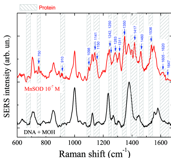
Figure 3: (red line) SERS spectrum of MnSOD after incubation of the functionalized nanoantenna dimers sample with a solution with protein at concentration 10^{-7}\text{ M} ( \lambda_{\text{exc}}=785\text{ nm} ). In addition to the spectral features arising from of the SERS of the functionalization layer (black line), we can see new peaks due to the protein whose position is labeled (highlighted by the dashed boxes). Spectra are shown after the continuum background removal and offset vertically for clarity reasons.
