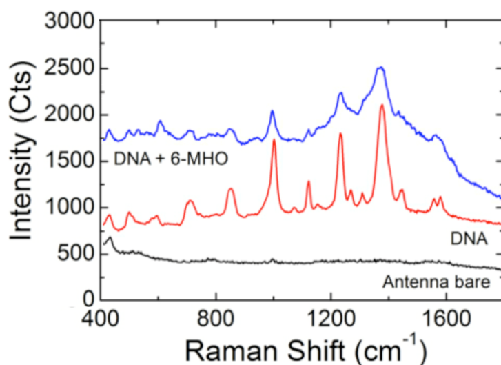
Figure 2: SERS spectra of the gold nanorods dimers ( \lambda_{exc}=785 nm) after ozone plasma cleaning (black line), after functionalization with thiolated DNA aptamers (red line) and after the addition of a further blocking layer of 6-MOH (blue line). Data are shown without any background subtraction.
