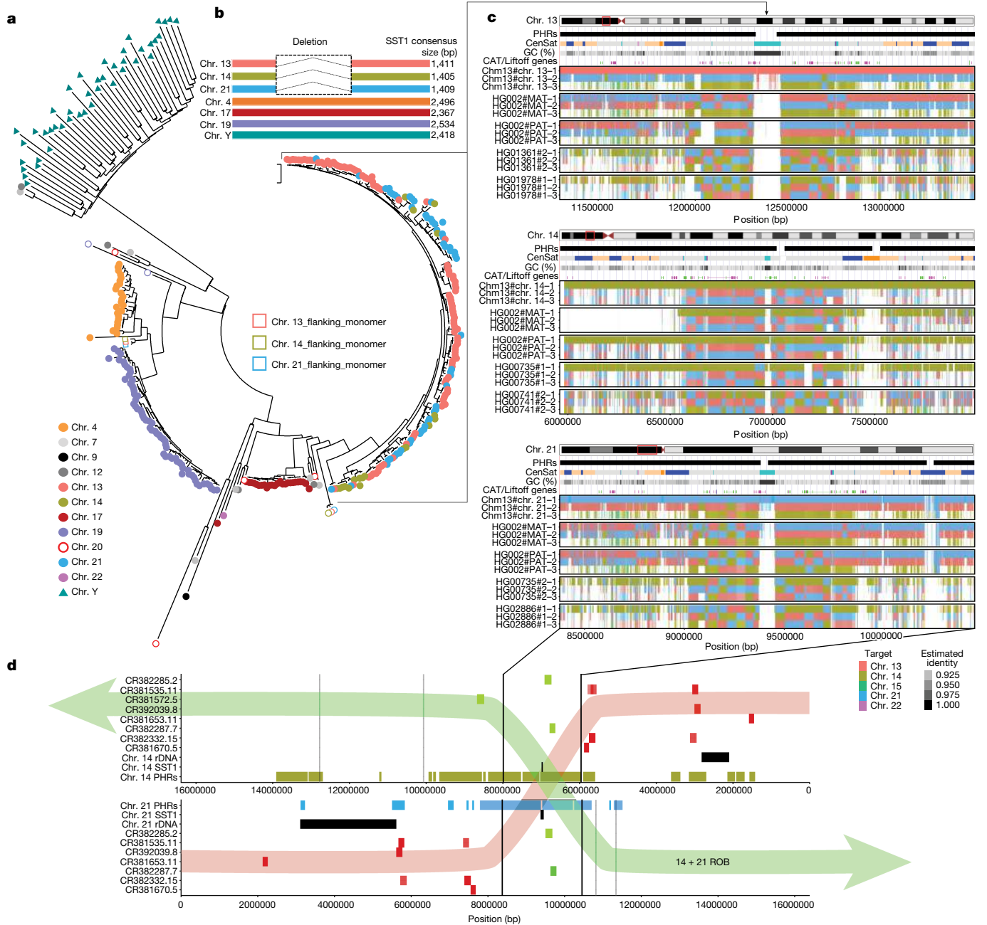
Fig. 4 | PHRs of chr. 13, chr. 14 and chr. 21, centred on the SST1 array. a , Maximum likelihood phylogenetic analysis of SST1 full-length elements indicates a recent homogenization process of acrocentric arrays. Coloured circles next to chromosome labels indicate individual monomers retrieved from the T2T-CHM13 assembly. Coloured triangles indicate SST1 full-length monomers retrieved from the HG002 chr. Y assembly. Partial or chimeric monomers flanking chr. 13, chr. 14 and chr. 21 arrays (located around 250 kb from the main array) are labelled as open circles or squares, respectively, coloured according to the corresponding chromosome. b , Schematic representation of SST1 consensus alignments, indicating a deletion that is present only in the SST1 unit from chr. 13, chr. 14 and chr. 21. c , Multiple untangling of T2T-CHM13, HG002-Verkko haplotypes and HPRCyl-acro contigs versus T2T-CHM13. Three of the five acrocentric chromosomes are represented. The degree of transparency indicates the estimated identity
