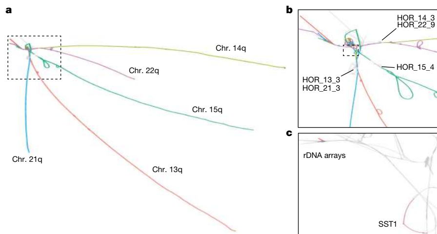
Fig. 2 | The acro-PVG derived from the HPRC1 assembly. a , The major component of the acro-PVG, shown with nodes in T2T-CHM13 chromosomes labelled with the colour scheme from Fig. 1a. The acrocentric q-arms are almost completely separated, whereas the p-arms unite in a tangle adjacent to the rDNA array. b , A close-up view of the SAAC junction, showing the separation of centromeric high-order repeats of chr. 15 (HOR_15_4) from the other chromosomes, whereas chr. 13 and chr. 21, and chr. 14 and chr. 22 share substantial homology in their arrays, which causes them to collapse in the PVG.
