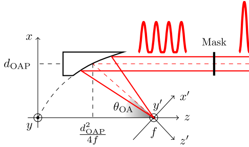
Fig. 2. Geometrical model. Cartesian coordinate system with the origin in the paraboloid vertex. The laser comes from the right and splits in 4 rings separated in time that will be focused on the focal plane x'y' .
