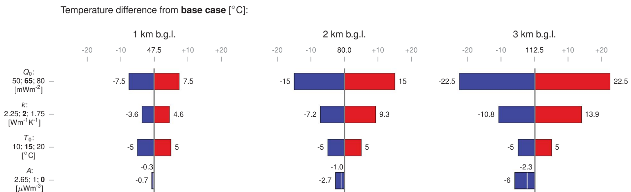
Fig. 2. Tornado plots showing the sensitivity of subsurface temperatures at three depth levels (1–3 km) to changes in surface heat flow ( Q_0 ), thermal conductivity ( k ), surface temperature ( T_0 ), and radiogenic heat production ( A ). For each parameter, three values are indicated that are used for the calculation. The values in bold are used to calculate default temperatures at each depth level. The other values are used to calculate temperature differences in respect to the default case.
