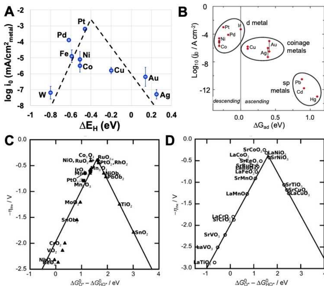
Figure 5. (A) Exchange current densities [ \log(i_0) ] on monometallic surfaces as a function of the calculated hydrogen binding energy. (B) Volcano curve for HER electrocatalysts at various metals in function of the energy of adsorption \Delta G_{ad} . OER theoretical overpotential vs. the differences between the standard free energy of two subsequent intermediates \Delta G_{O^*}^0 - \Delta G_{HO^*}^0 considering (C) various binary oxides and (D) perovskite oxide. (A) Reproduced with permission from Ref. [97]; copyright 2013, Royal Society of Chemistry. (B) Adapted from Ref. [98] under CC BY 4.0 ( https://creativecommons.org/licenses/by/4.0/ ). (C,D) Adapted with permission from Ref. [99]; copyright 2011, Wiley-VCH.
