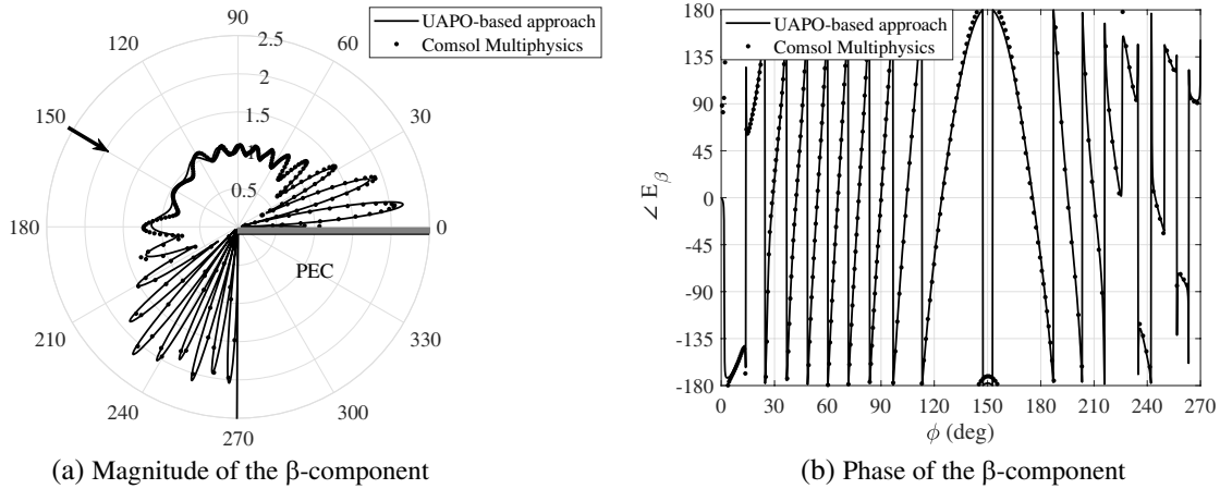
Figure 6. Magnitude and phase of the field \beta -component when \beta' = 90^\circ , \phi' = 150^\circ and E_{\beta'}^i = 1 , E_{\phi'}^i = 0 . DNG MTM coating with d = 0.1\lambda_0 , \mu_r = -1 , \epsilon_r = -(4 + j0.01) .
