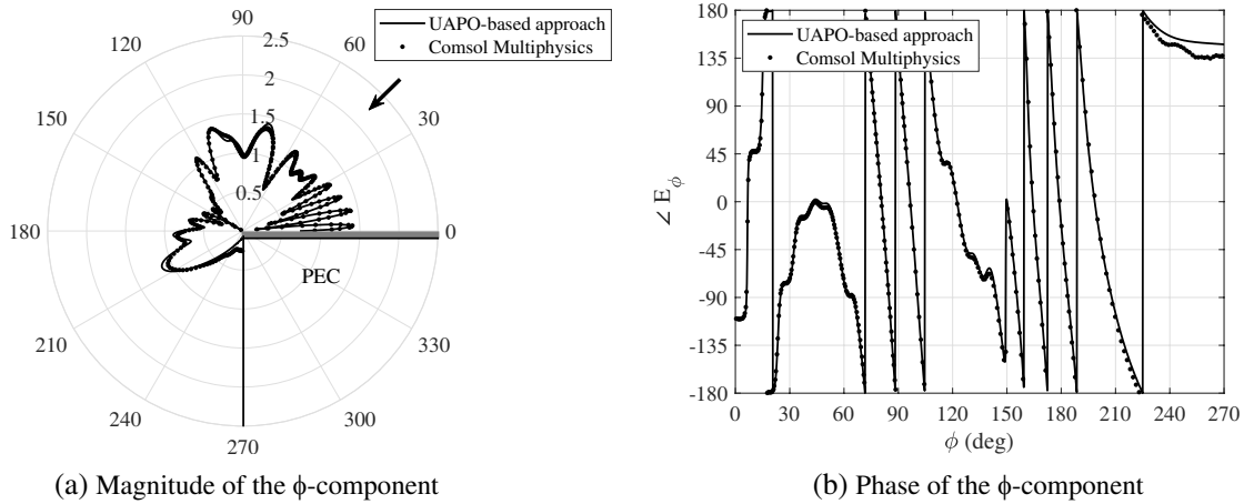
Figure 5. Magnitude and phase of the field \phi -component when \beta' = 90^\circ , \phi' = 45^\circ and E_{\beta'}^i = 0 , E_{\phi'}^i = 1 . DNG MTM coating with d = 0.1\lambda_0 , \mu_r = -1 , \epsilon_r = -(4 + j0.01) .
