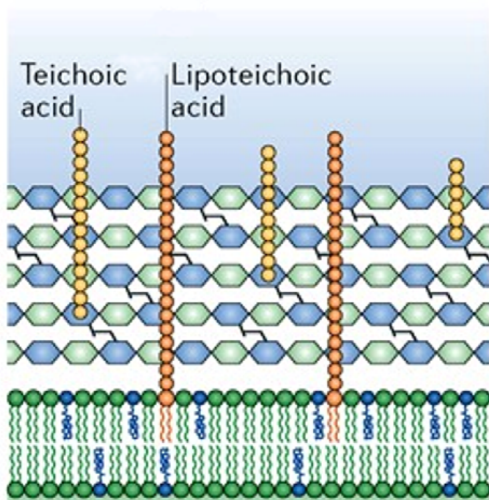
Gram-positive bacteria
