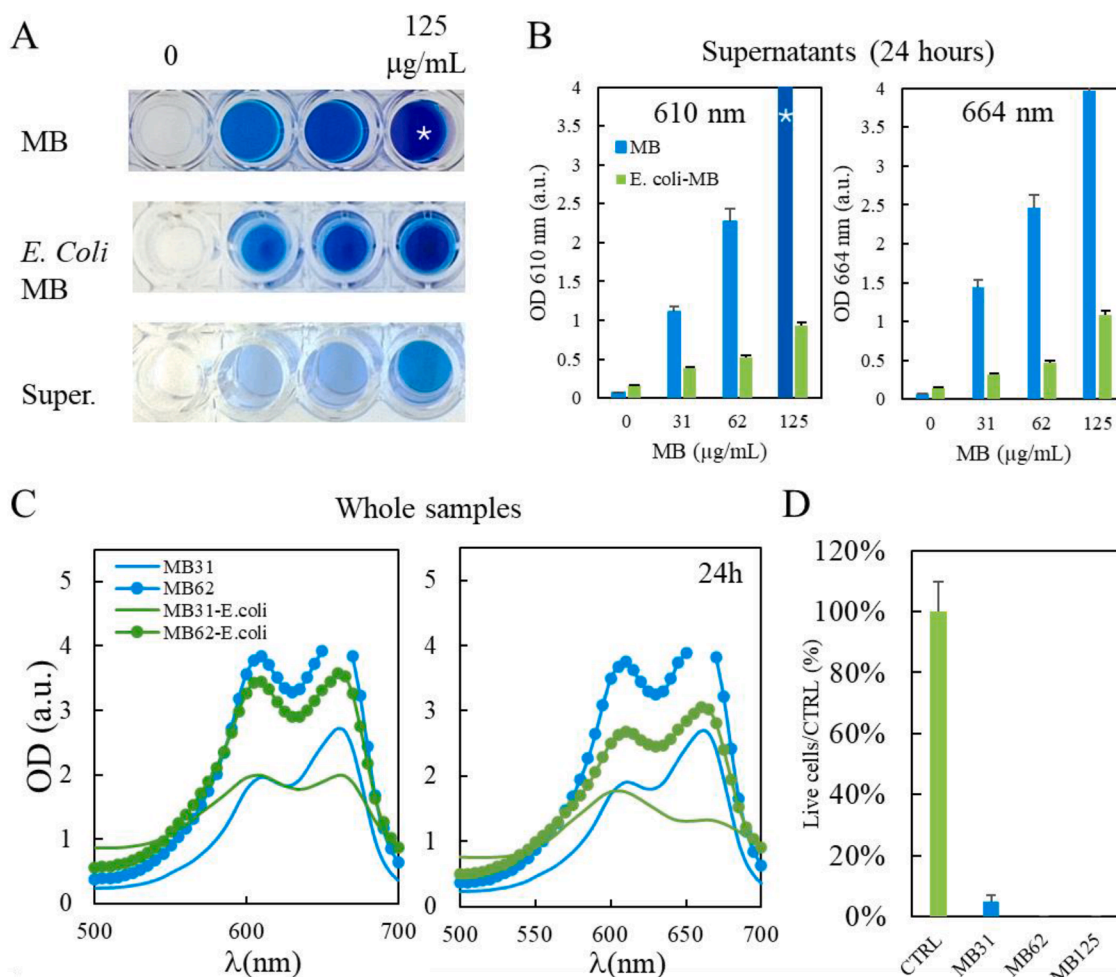
Fig. 2. Interaction of MB with E. coli after 24 h incubation. (A) Representative images of MB solutions at increasing concentrations (0–125 µg/mL) in the absence and presence of E. coli , before and after centrifugation. The formation of a blue pellet indicates MB association with bacterial cells. (B) Quantification of MB in supernatants after centrifugation, showing a concentration-dependent decrease in absorbance at 610 nm and 664 nm in the presence of E. coli , without significant changes in their ratio. (C) UV-Vis absorption spectra of whole samples at 0 h and after 24 h incubation. In the presence of E. coli , a decrease of the 664 nm band and a blue shift with increased intensity and broadening of the ~610 nm band are observed, consistent with the formation and stabilization of aggregated Mb species . (D) CFU results obtained treating cells with increasing MB concentration.
