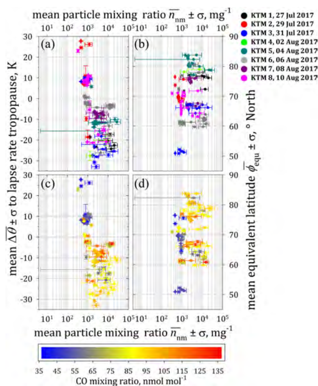
Figure 6. Mean particle mixing ratio \bar{n}_{nm} of individual NPF events as a function of (a, c) the vertical distance from the mean lapse-rate tropopause ( \overline{\Delta\theta} ) and of (b, d) the equivalent latitude ( 90^\circ represents the centre of the AMA as projected to polar coordinates). Data points are coloured by flight date (a, b) and by CO mixing ratios (c, d). (e) The mean particle mixing ratio \bar{n}_{nm} as a function of the equivalent latitude is colour-coded by the values \overline{\Delta\theta} (colour scale on the left of panel e).
