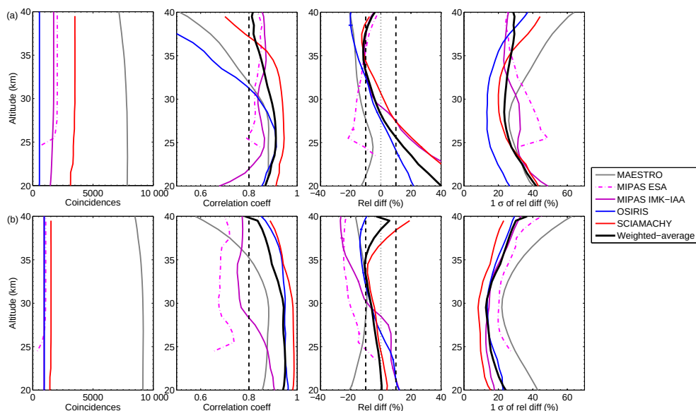
Figure 8. Comparisons of ACE-FTS NO 2 profiles with correlative data sets using coincidence criteria of within 4 h and 350 km: (a) comparisons for local morning and (b) local evening. Note that GOMOS and the solar occultation instruments have been excluded. Error bars in the relative difference profiles represent the standard error of the mean (values less than ~ 1 % may not be visible).
