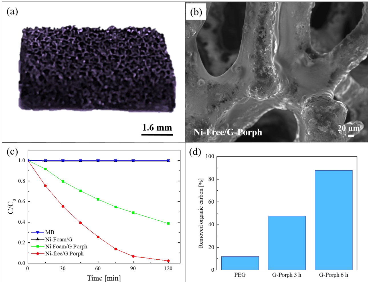
Figure 9. (a) Photograph of Ni-Free/G-Porph sample; (b) SEM image of Ni-Free/G-Porph sample; (c) photocatalytic activity of Ni-Foam/G, Ni-Foam/G-Porph, Ni-Free/G-Porph toward the degradation of MB; (d) Total organic carbon (TOC) measurements of pristine PEG after 6 h of irradiation, and in the presence of Ni-Free/G-Porph after 3 and 6 h of irradiation, respectively [78].
