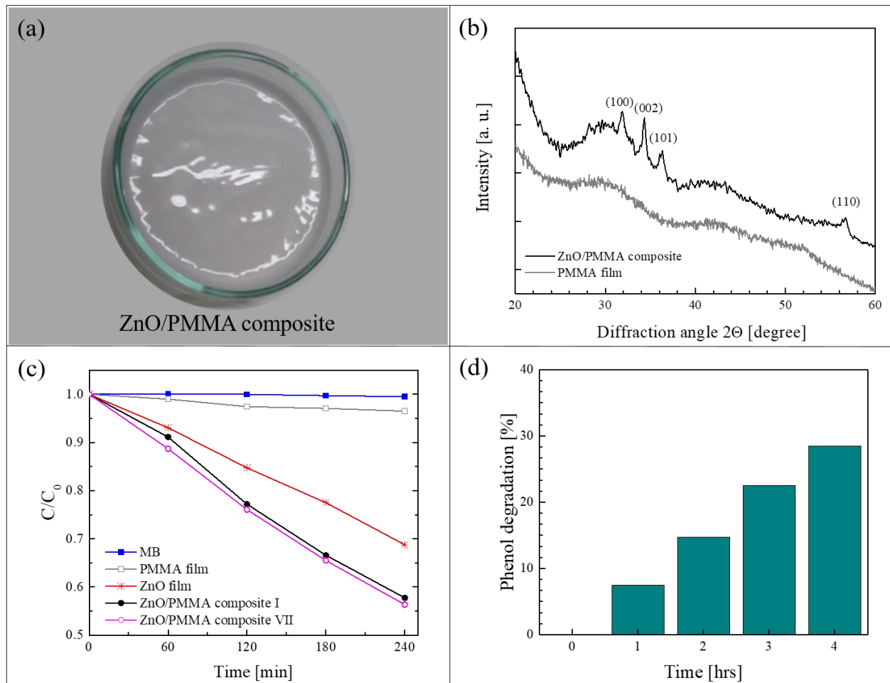
Figure 5. (a) Photo of ZnO/PMMA sample in a Petri dish; (b) X-ray diffraction (XRD) patterns of PMMA film and of ZnO/PMMA composite film; (c) MB photodegradation under UV light in the presence of PMMA film, ZnO/Si film, ZnO/PMMA film, the discoloration of pure MB and the photocatalytic activity of the ZnO/PMMA film after seven cycles are reported too; (d) phenol photodegradation under UV light in the presence of ZnO/PMMA film [64].
