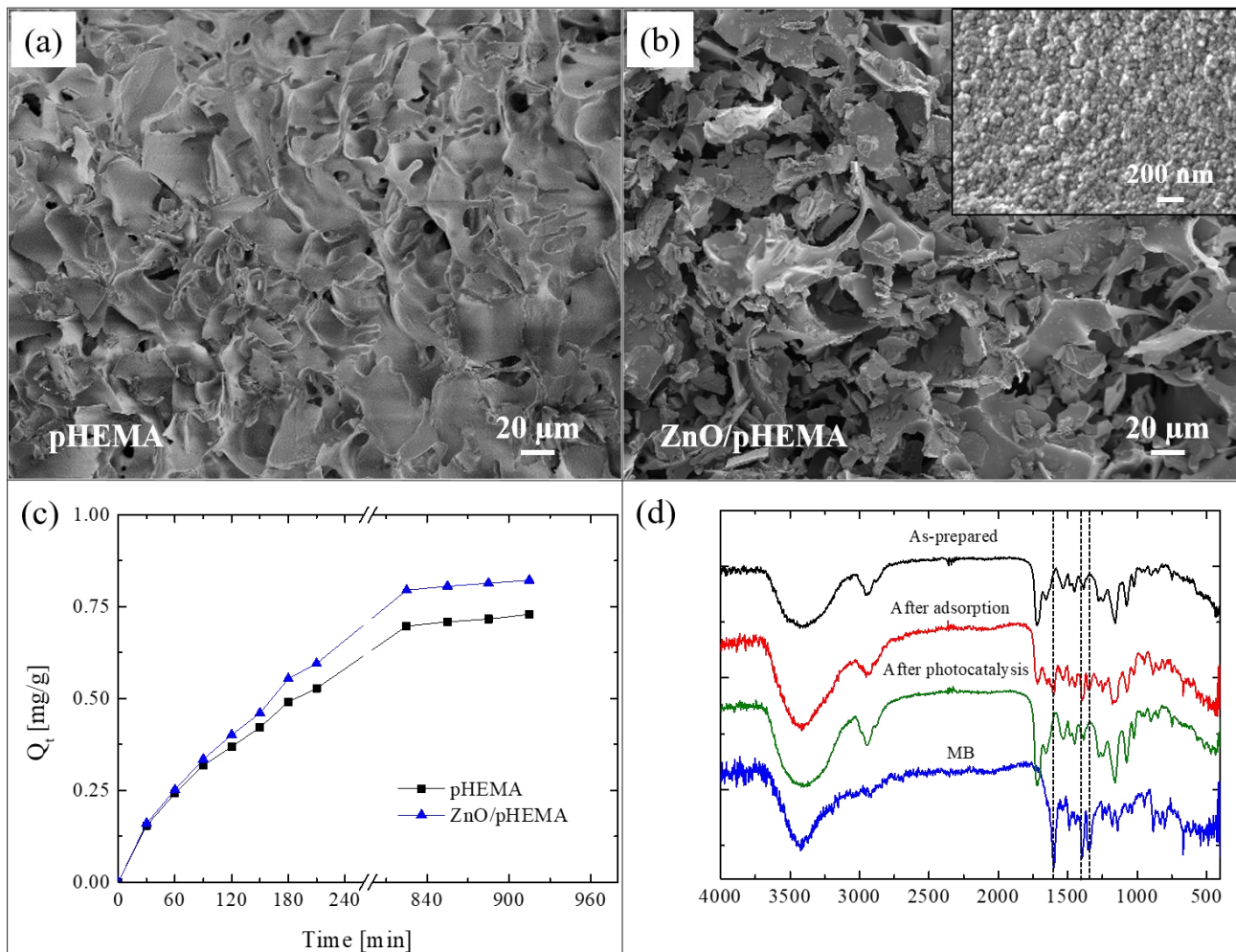
Figure 10. (a) SEM image of poly(2-hydroxyethylmethacrylate) (pHEMA) sample; (b) SEM image of ZnO/pHEMA sample; (c) MB adsorption capacity versus time for pHEMA and ZnO/pHEMA samples; (d) Fourier transform infrared spectroscopy (FTIR) spectra measured on ZnO/pHEMA samples: as-prepared, after MB adsorption, and after UV light irradiation; the spectrum of pure MB is also reported as reference [81].
