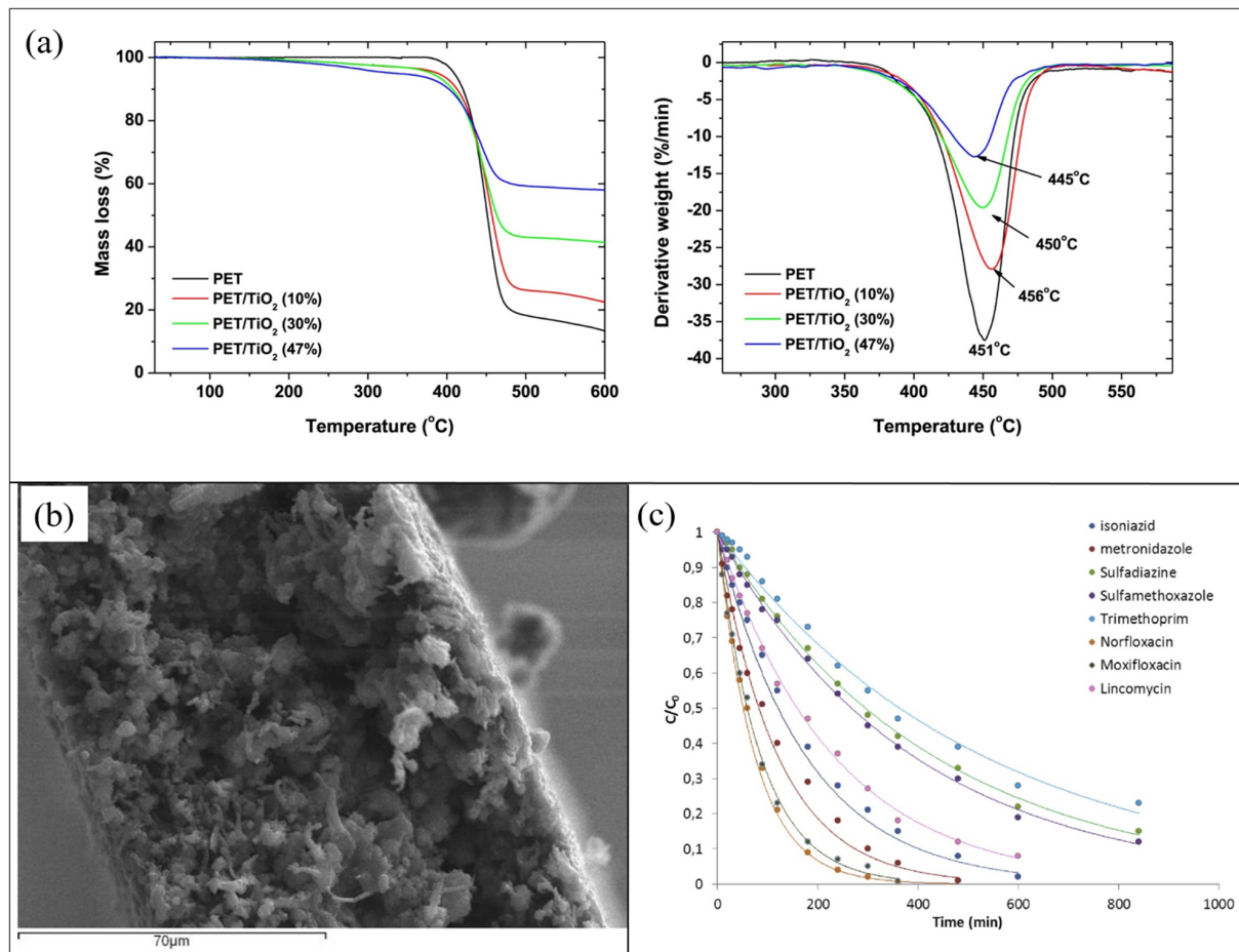
Figure 2. (a) Mass loss and derivative weight curves of composite films containing different \text{TiO}_2 contents; (b) SEM image of poly(ethylene terephthalate) (PET) with 10 wt% \text{TiO}_2 ; (c) photocatalytic degradation of antibiotics in the presence of PET 10 wt% \text{TiO}_2 composite films in a wastewater effluent. Figure 2 was adapted from [55], with the permission of Elsevier.
