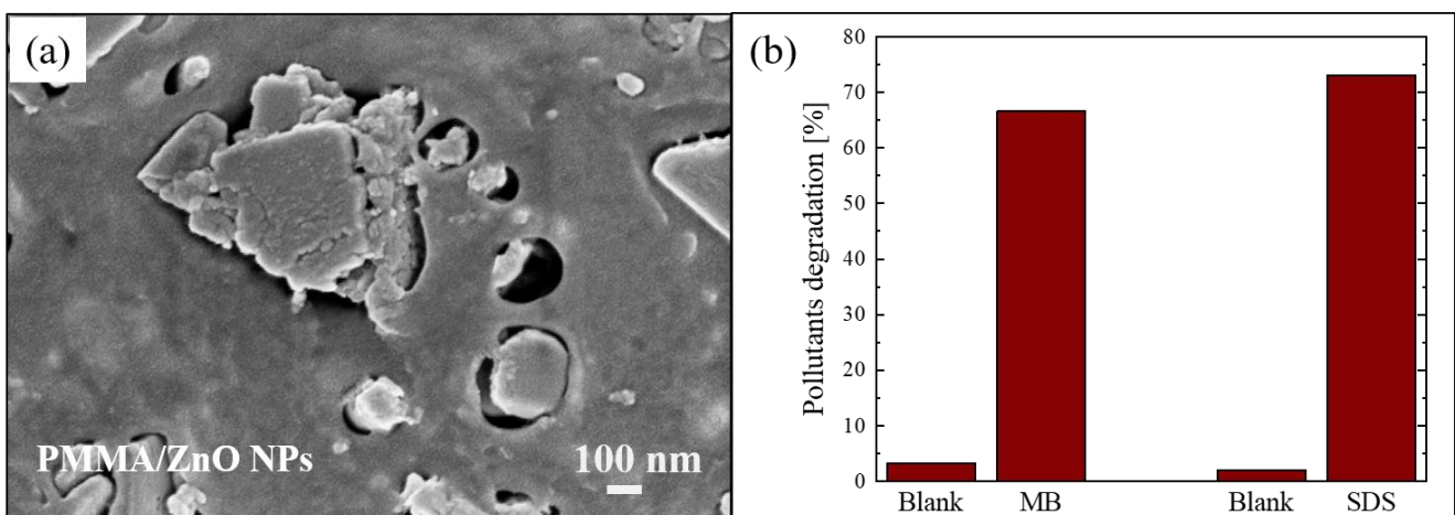
Figure 4. (a) Plan-view SEM image of the back surface of PMMA/ZnO NPs sample; (b) MB and sodium dodecyl sulfate (SDS) degradation under UV irradiation for 4 h in the presence of PMMA/ZnO NPs sample [61].
