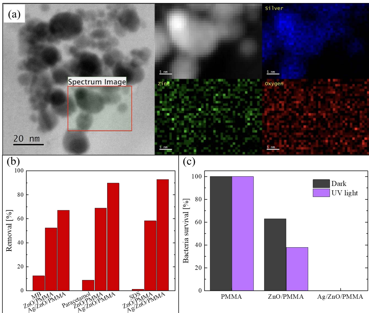
Figure 6. (a) Scanning transmission electron microscopy (STEM) image of Ag NPs on the ZnO surface and energy-dispersive X-ray spectroscopy (EDS) signals from silver, zinc, and oxygen; (b) degradation of MB, paracetamol, and SDS after 4 h under UV irradiation for blank solutions, in the presence of ZnO/PMMA, and in the presence of Ag/ZnO/PMMA; (c) bacterial survival percentage in the dark and when exposed to UV irradiation for 1 h in contact with PMMA, ZnO/PMMA, and Ag/ZnO/PMMA samples [65].
