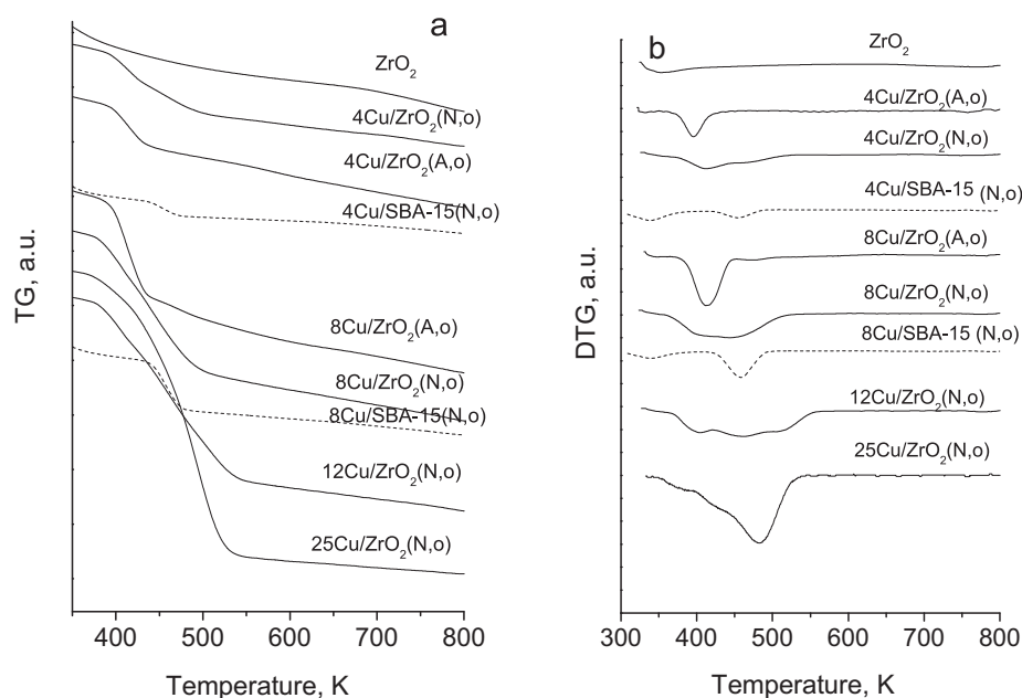
Fig. 5. TPR-TG (left) and TPR-DTG (right) profiles of pure ZrO_2 and its copper modifications. For comparison, selected TPR profiles of SBA-15 silica based modifications are also shown.
