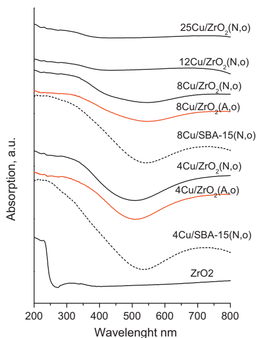
Fig. 3. UV-vis spectra of copper modifications of ZrO 2 . For comparison, the spectra of selected copper modified SBA-15 are also presented (dash lines).
