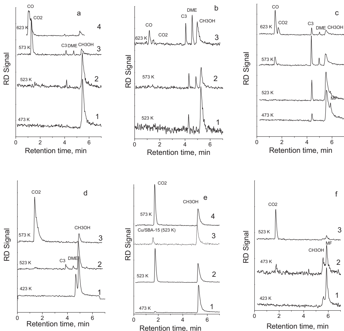
Fig. 8. ^{11}\text{CH}_3\text{OH} decomposition at various temperatures on: \text{ZrO}_2 after procedure A (a), \text{ZrO}_2 after procedure B (b), 8\text{Cu}/\text{ZrO}_2(\text{N},\text{o}) after procedure A (d) and 8\text{Cu}/\text{ZrO}_2(\text{N},\text{o}) after procedure B (e). ^{11}\text{CH}_3\text{O}-\text{CHO} decomposition after procedure C on \text{ZrO}_2 (c) and 8\text{Cu}/\text{ZrO}_2(\text{N},\text{o}) (f).
