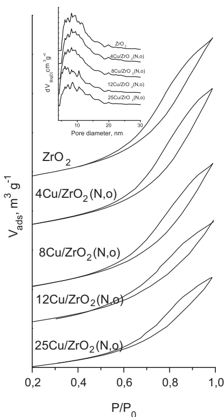
Fig. 1. Nitrogen physisorption isotherms and pore size distribution (inset) for ZrO_2 and various copper zirconia modifications.
