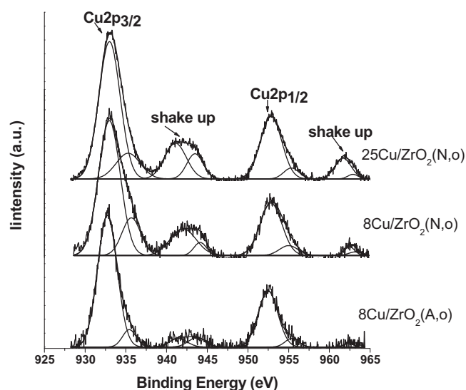
Fig. 4. Cu 2p photoelectron spectra of selected samples.
