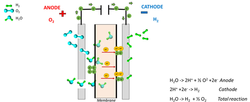
Figure 1. Working principle of a PEM electrolyzer.
