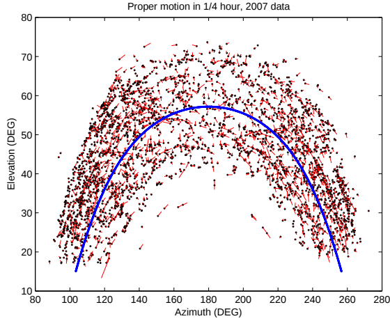
Figure 3. Validation dataset: 2007 tracklets from ESA OGS, pre-processed by University of Bern. Angles are in a body-fixed altazimutal reference. Angular velocity is represented by the motion in 1/4 hour. The blue line is the geostationary line (where GEO with e = I = 0 are found).
