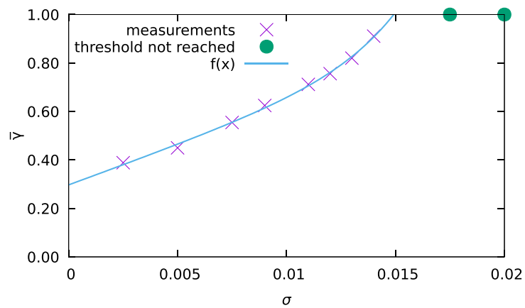
Figure B3. \bar{\gamma} versus the noise amplitude \sigma . The green circles represent \sigma values for which \rho(\sigma) = 0.5 was never reached. The blue solid line is a fit to the data (violet crosses) performed via the expression (36), the fit is employed to extrapolate the critical noise value \sigma_c for which \rho(\sigma_c, \bar{\gamma} = 1) = 0.5 . Other parameters as in figure B2 apart B = 192 .
