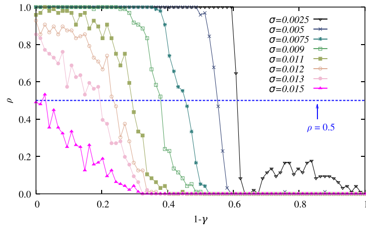
Figure B2. Stability parameter \rho versus 1 - \gamma , where \gamma is the modulation factor entering in (23). For each measurement of \rho we averaged over B = 96 different noise realisations and each time we estimated \Sigma_v from a time series of duration T_W = 0.3 s after discarding a transient T_t = 16 s. The dashed line indicates \rho = 0.5 , i.e. where the system has an equal probability to end in the asynchronous or clustered state. The data refer to a system size N = 32\,000 , other parameters as in figure B1.
