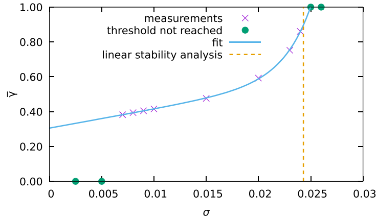
Figure 8. \bar{\gamma} versus the noise amplitude \sigma . The green circles represent \sigma values for which \rho(\sigma) = 0.5 was never reached. The blue solid line is a fit to the data (violet crosses) performed via the expression (36), the fit is employed to extrapolate the critical noise value \sigma_c for which \rho(\sigma_c, \bar{\gamma} = 1) = 0.5 . The vertical dashed line shows the mean-field prediction \sigma_H for the onset of COs. Errorbars are omitted since the errors are smaller than symbol size. Other parameters as in figure 7 apart the number of different realisations, that now is M = 384 .
