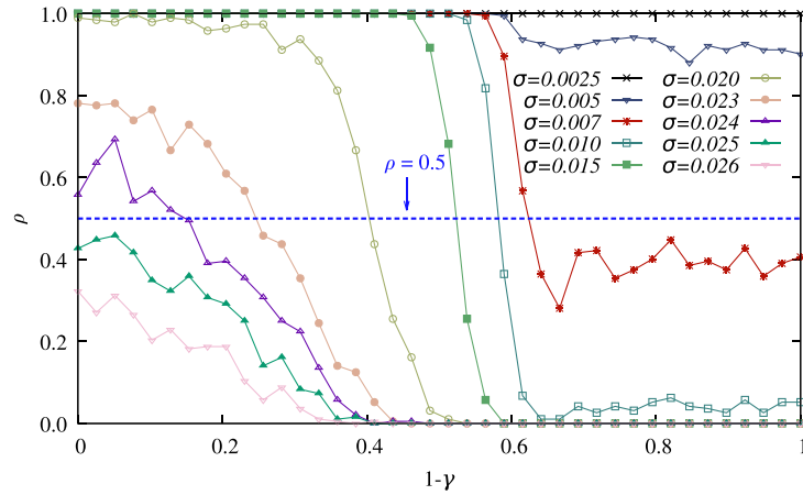
Figure 7. Stability indicator \rho versus 1 - \gamma , where \gamma is the factor entering in (23). For each measurement of \rho we considered M = 192 different realisations and each time we estimated \Sigma_v from a time series of T_W = 0.3 s after discarding a transient T_t = 16 s to evaluate if the system remains asynchronous or becomes clustered. The dashed line indicates \rho = 0.5 , i.e. where the system has an equal probability to move towards either the asynchronous or the clustered state. The data refer to a system size N = 32000 , other parameters as in figures 1(b) and (c).
