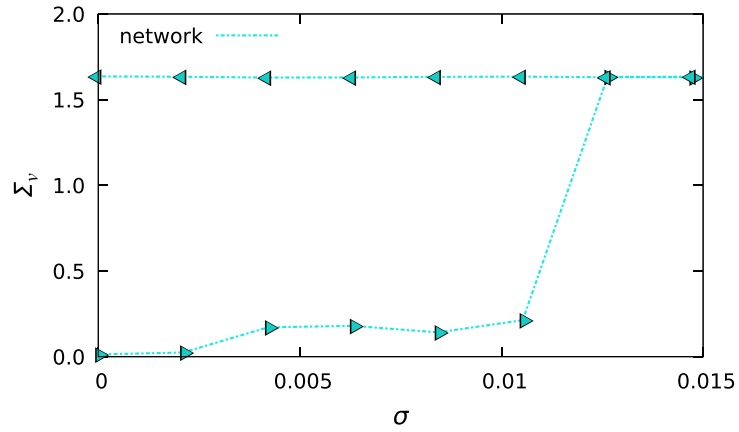
Figure B1. Variance \Sigma_v of the mean membrane potential v versus noise amplitude \sigma obtained via quasi-adiabatic simulations. The decrease or increase of the noise amplitude \sigma performed during the adiabatic simulations is indicated by the direction of the triangles' tip. The dashed lines are simply intended as a visual aid. The parameters for the quasi-adiabatic simulations are \Delta\sigma = \frac{0.4}{19} , t_T = 20 s, t_S = 25 s. The other parameters are set as in figure 2 with \Delta_J = 0 for a network size N = 200\,000 .
