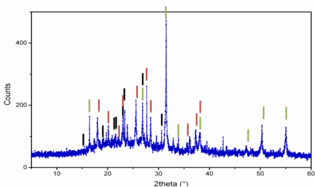
Figure 4. Diffraction pattern of a part of the grisaille of fragment SSGP1. The positions of the diffraction peaks of the spinel \text{CoAl}_2\text{O}_4 (green), laurionite \text{PbCl(OH)} (black) and Anglesite \text{PbSO}_4 (red) are indicated.
