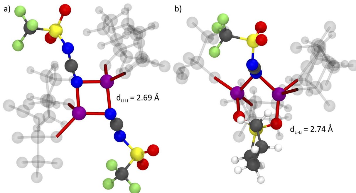
Fig. 13 Bridging coordination patterns found in the MD simulation of [Li(SL) 2 ][TfN(CN)], (a) involving two anions and (b) involving one anion and one sulfolane molecule. Lithium atoms are shown in purple. For each lithium atom, the four close contacts to the coordination partners are highlighted in red. Coordinating molecules not participating in bridging coordination are shown as ghosts. The colour code for the other atoms is blue – nitrogen, grey – carbon, yellow – sulphur, red – oxygen, green – fluorine.
