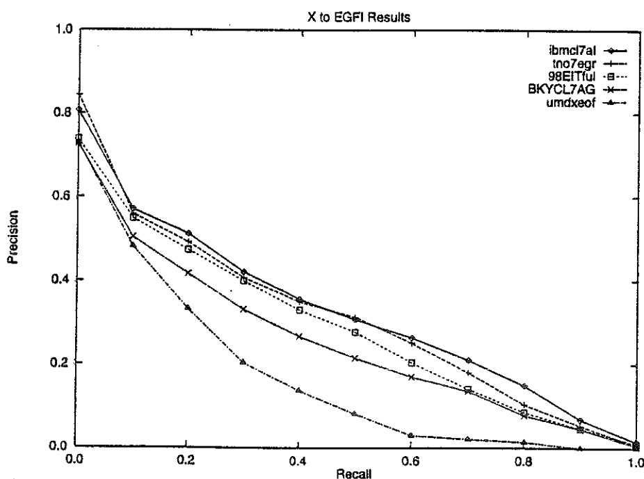
Figure 2: Results of the main evaluation X \rightarrow EGFI .
