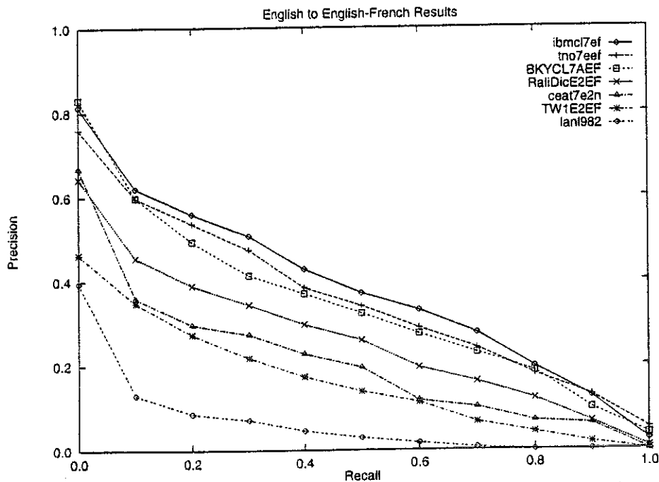
Figure 3: Results of the secondary evaluation E→EF.
