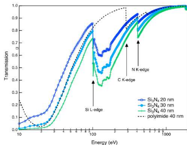
Fig. 1 Comparison of the calculated transmission of 40 nm of polyimide (black dashed line), 40 nm of \text{Si}_3\text{N}_4 (green solid line), 30 nm of \text{Si}_3\text{N}_4 (light blue solid line), and 20 nm of \text{Si}_3\text{N}_4 (dark blue solid line).
