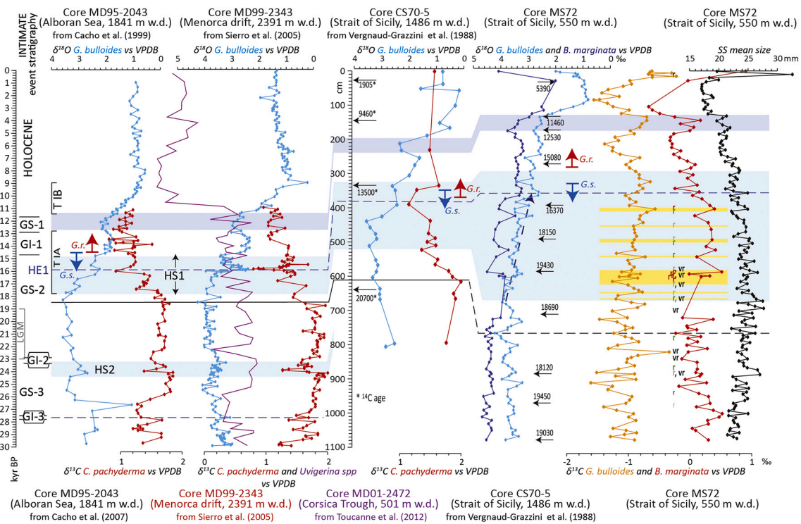
Fig. 11. Basin-wide correlation of benthonic and planktonic \delta^{13}\text{C} and \delta^{18}\text{O} records of core MS72 and the reference cores of the Mediterranean (see references on top of each core). The ages are calibrated (yr BP). The yellow stripes represent the intervals with evidence of major reworking/displacement of foraminifera. See Fig. 7 for a detailed explanation of symbols and abbreviations. (For interpretation of the references to colour in this figure legend, the reader is referred to the web version of this article.)
