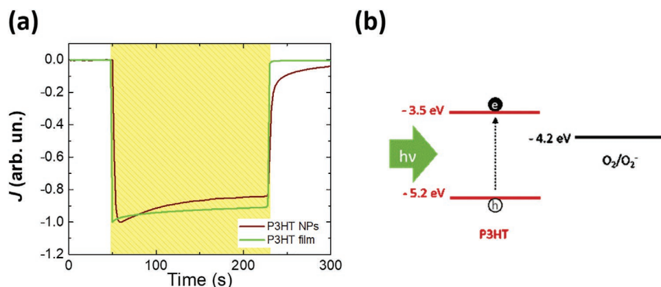
Figure 5. Photocathodic current generation by P3HT NPs dispersion. a) Comparison among photocurrent ( J ) signals (normalized to the maximum absolute J values) obtained in P3HT NPs dispersion and P3HT thin films spin-coated from solution onto the ITO slab. Photoexcitation is represented by the yellow-shaded area (LED emission wavelength peak, 470 nm; stimuli duration, 3 min; photoexcitation density, 2.7 \text{ mW mm}^{-2} ). b) P3HT HOMO/LUMO energetic levels are compatible with oxygen reduction reactions occurring at the polymer/electrolyte interface.
