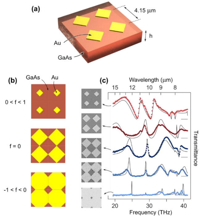
Fig. 1. Schematic of the complementary metasurface family and transmission spectra. a) Details of the metasurface in a 3d rendering. b) Top-view of four unit cells with indication of the ranges of the parameter f that identifies connected/disconnected metallic patterns. f = 0 is the self-complementary structure. c) Measured (colored dotted traces) and calculated (solid black lines) transmission spectra of five fabricated samples, with f = -0.54, -0.29, -0.035, 0.23, 0.45 (from bottom to top). The corresponding scanning electron micrographs are also reported. The measured data are scaled and offset by arbitrary factors, while the calculated traces are absolute transmittance values and are offset by one unit.
