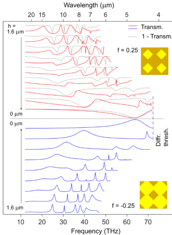
Fig. 3. Recovery of Babinet theorem in a series of complementary metasurfaces supported by dielectric slabs of different thicknesses h . ( h = 1.6, 1.4, 1.2, 1, 0.8, 0.6, 0.4, 0.2, 0 \mu\text{m} ). As the slab thickness approaches zero, complementary transmission spectra are observed. The spectra (absolute transmittance) are offset by 1.2 units.
