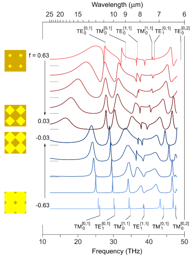
Fig. 2. Violation of Babinet theorem observed in a series of complementary slab-supported metasurfaces. The transmittance spectra (absolute transmittance, each offset by 0.8) do not comply with the Babinet theorem requirement T(v; f) = 1 - T(v; -f) , where v is the frequency and f is the complementarity-controlling geometrical parameter. The labels \text{TE}_j^{[mn]} and \text{TM}_j^{[mn]} identify the guided mode resonances originating from the slab waveguide modes. A detailed analysis is provided in the main text.
