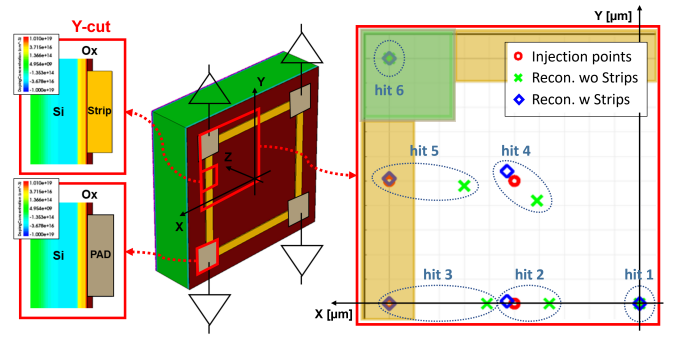
Figure 2: Left side, layout of the simulated DC-RSD structure with strip-connected pads and cuts along the sensor depth, which show the direct coupling of the resistive silicon layer to the read-out pads (grey) and the strips (orange). Right side, detail of the upper left quadrant of the map of the injected (red circular markers) and reconstructed (blue diamond and green cross markers) particle impact positions. Six injection points (hits) have been tested in the case of DC-RSD flavor without strips (wo Strips) and strip-connected one (w Strips).
