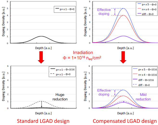
Figure 1: Evolution with irradiation of a simulated gain layer profile (Gaussian) in standard (left) and compensated (right) LGAD, after a fluence of 1 \cdot 10^{16} n_{eq}/cm^2 . In the compensated design, four parts of an n^+ -dopant are used to balance five parts of the p^+ one. Their difference (diff) results in an effective doping concentration similar to that of the standard LGAD before the irradiation, but in an almost unchanged one after the irradiation.
