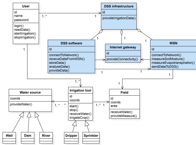
(a) UML class diagram
