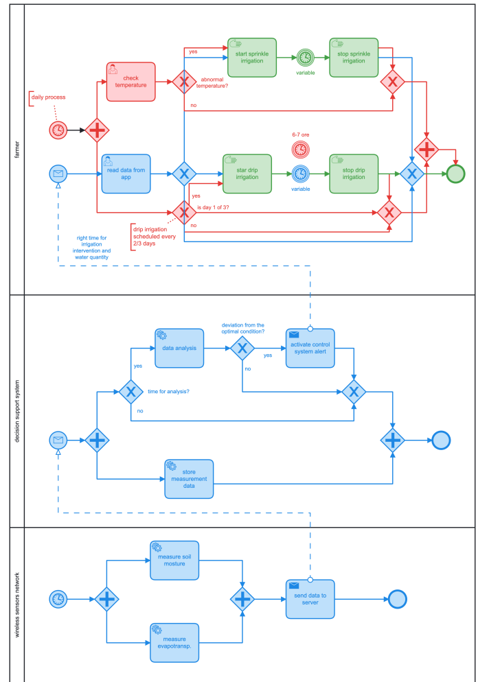
(c) comparison of BPMN process diagrams
