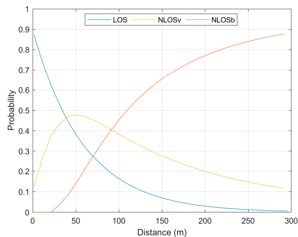
Figure 2. Probabilities of LOS, NLOS v , and NLOS b propagation conditions along the optical path between a transmitting car and a road user in urban settings as a function of the distance d_i from the transmitting car.
