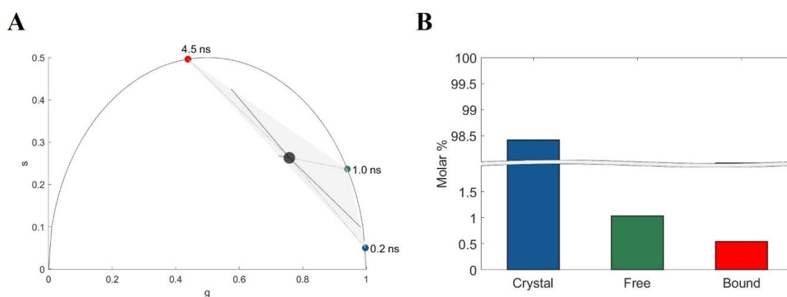
Figure 2: Phasor analysis of standard liposomal doxorubicin. A) Graphical calculation of fractional-intensity contributions. Dotted lines connect each pure species to the experimental phasor and are extended as a continuous line to the edge joining the other two pure species. Equation 1 determines the fractional intensity. B) Resulting molar fractions in Doxoves® after the application of Equation 2. Crystal DOX is 98.419 \pm 0.005 , free DOX 1.036 \pm 0.005 and lipid-bound DOX is 0.545 \pm 0.001 .
