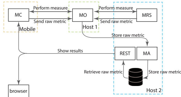
Fig. 3: Validation setup
