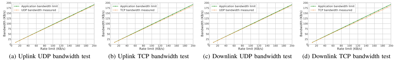
Fig. 5: Validation tests for UDP and TCP bandwidth estimation mechanisms.
