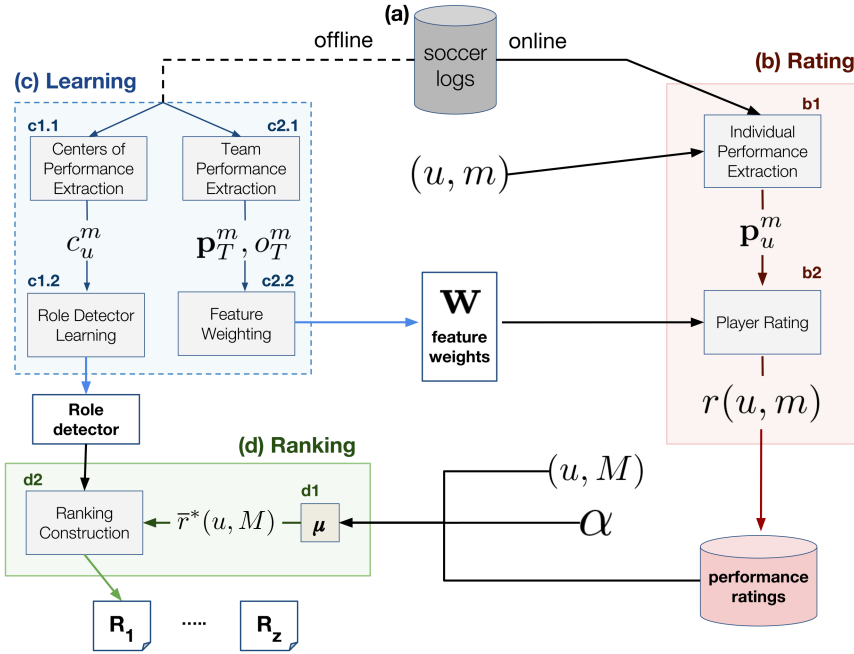
Fig. 1. Schema of the PlayRank framework. Starting from a database of soccer-logs (a), it consists of three main phases. The learning phase (c) is an “offline” procedure: It must be executed at least once before the other phases, since it generates information used in the other two phases, but then it can be updated separately. The rating (b) and the ranking phases (d) are online procedures, i.e., they are executed every time a new match is available in the database of soccer-logs. We refer to the text for the notation used in the figure.
