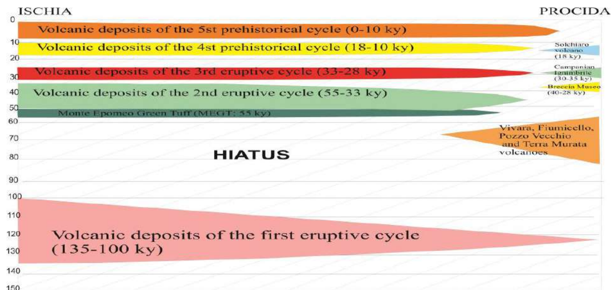
Figure 16. Qualitative chronostratigraphic diagram of Ischia. The decrease in triangles is due to the decrease in the thickness of the volcanic deposits.
