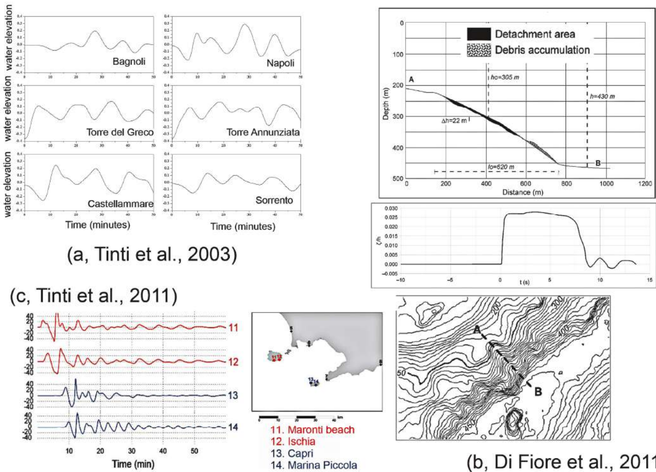
Figure 8. Mareograms related to tsunami in Naples Bay ((a), modified after Tinti et al. [19]), ((b), modified after Di Fiore et al. [41]), and Ischia ((c), modified after Tinti et al. [20]). In sub-figure (b), h_0 is the characteristic water depth, h is the water depth, and \zeta is the free surface displacement. In sub-figure. AB is the bathymetric profile. (c), the modeled tsunami refers to Ischia as controlled by the Ischia debris avalanche (IDA) [15].
