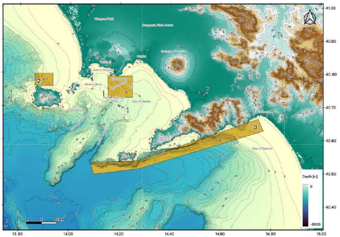
Figure 2. Digital elevation model of Naples Bay showing the location of study areas (1: Ammontatura slope basin and the northern branch of the Dohnr canyon; 2: northern Ischia debris avalanche deposits; 3: southern slope of the Sorrento Peninsula).
