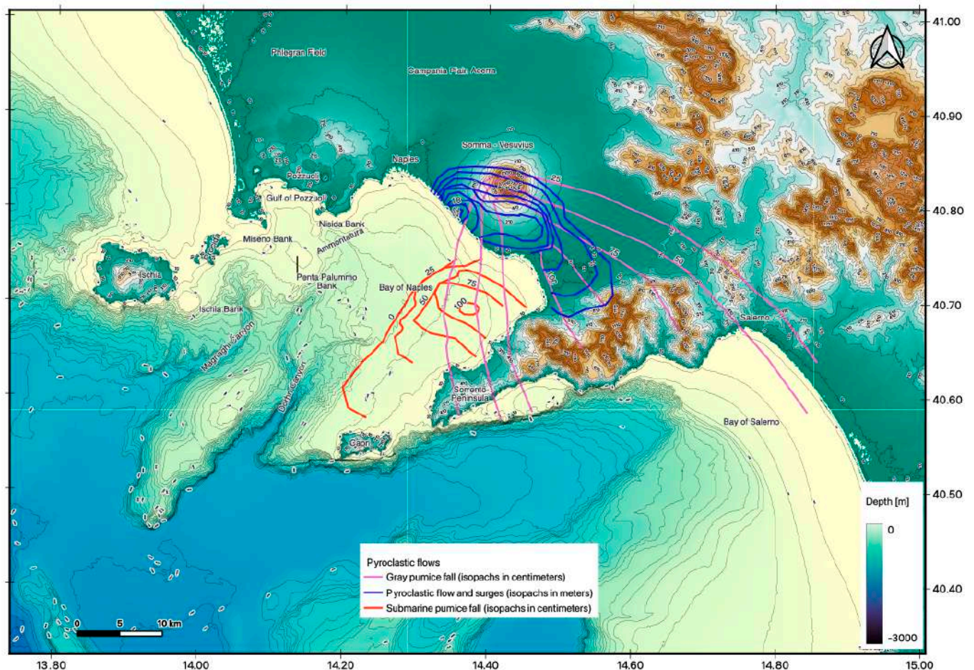
Figure 7. Pyroclastic flows related to the AD 79 eruption in Naples Bay (modified after Milia et al. [63]).
