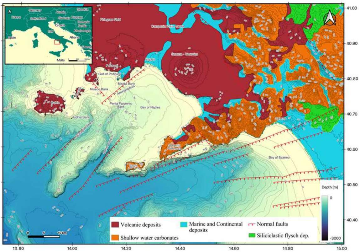
Figure 1. Geologic sketch map of the Bay of Naples and the surrounding emerged areas.
