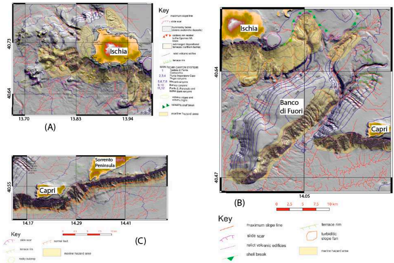
Figure 15. Detailed geomorphological maps of Naples Bay showing marine hazards (in yellow). (A) Ischia; (B) Naples canyons, (C) southern slope of the Sorrento Peninsula (modified after Aiello and Sacchi [24]).
