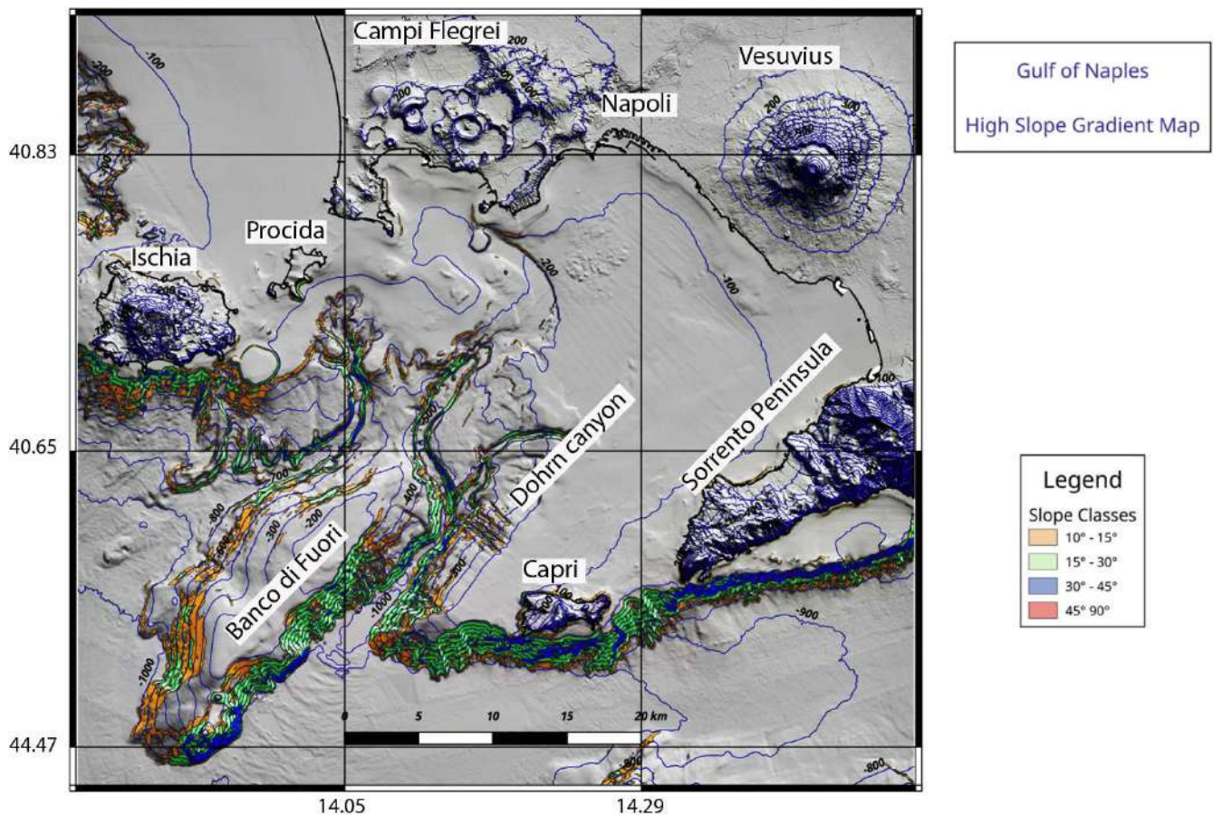
Figure 4. High-slope map of Naples Bay, showing marine areas potentially prone to slide (modified after Aiello and Sacchi [24]).
