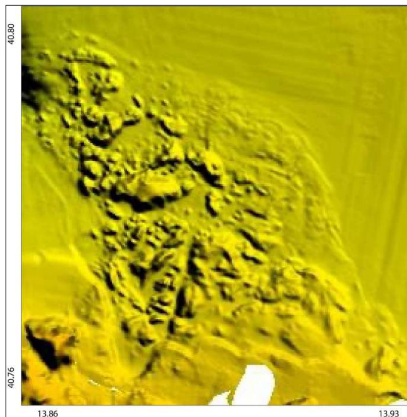
Figure 12. Detailed DEM of the northern Ischia debris avalanche.
