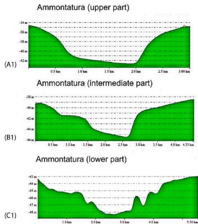
Figure 9. Detailed DEM and bathymetric profiles of the Ammontatura slope basin (modified after Aiello et al. [16]) A–D/A1–C1 indicate the bathymetric profiles.
