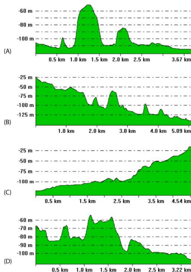
Figure 13. Bathymetric profiles in the northern Ischia debris avalanche deposits (A–D) represent the bathymetric profiles.
