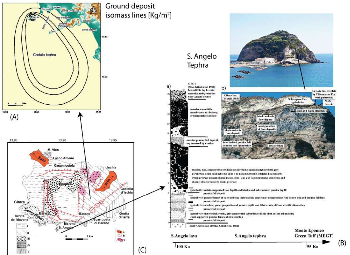
Figure 5. (A) Ground deposit isomass lines (kg/m 2 ) on domain covered by Cretaio tephra (Tyrrhenian Sea; modified after Primerano et al. [50]). (B) S. Angelo tephra of Ischia (modified after Brown et al. [45]) (a) Sketch stratigraphic column of the tephra. (b) Significant outcrop of the S. Angelo tephra. (C) Location of the Cretaio and S. Angelo tephra superimposed on the geological map of Ischia. Key. I scree and mud flows; II volcanic units younger than 10,000 years; III older volcanic rocks (between 20,000 and 33,000 years ago); IV GreenTuff of Mount Epomeo; V first volcanic complex, now dismantled (including the first and the second phase of Ischia activity).
