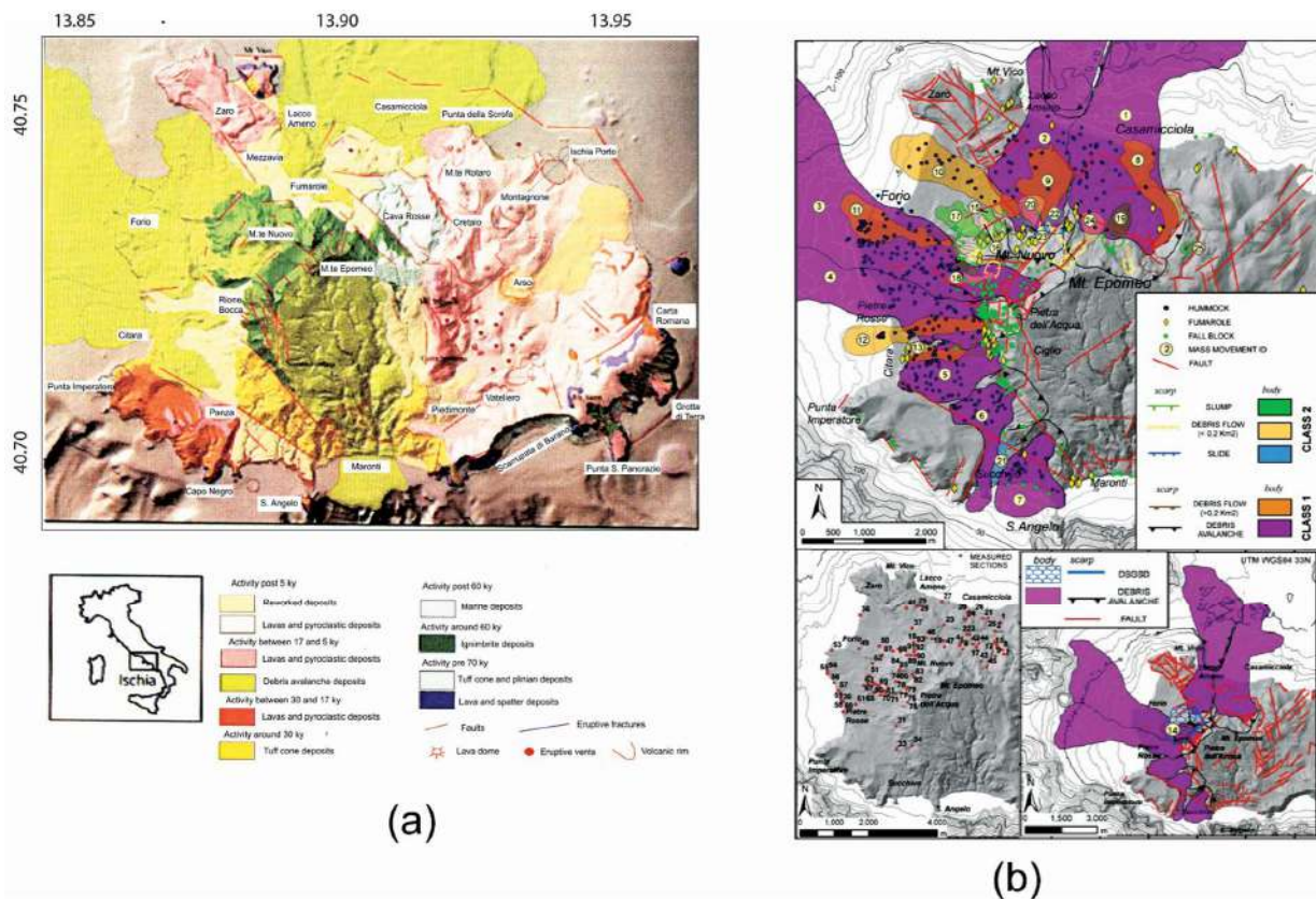
Figure 3. (a) Geologic sketch map of Ischia (modified after Sbrana et al.) [37]. (b) Onshore and offshore extension of the Epomeo Mt. gravitational landforms and offshore extension of the debris avalanche deposits (modified after Della Seta et al.) [38].
