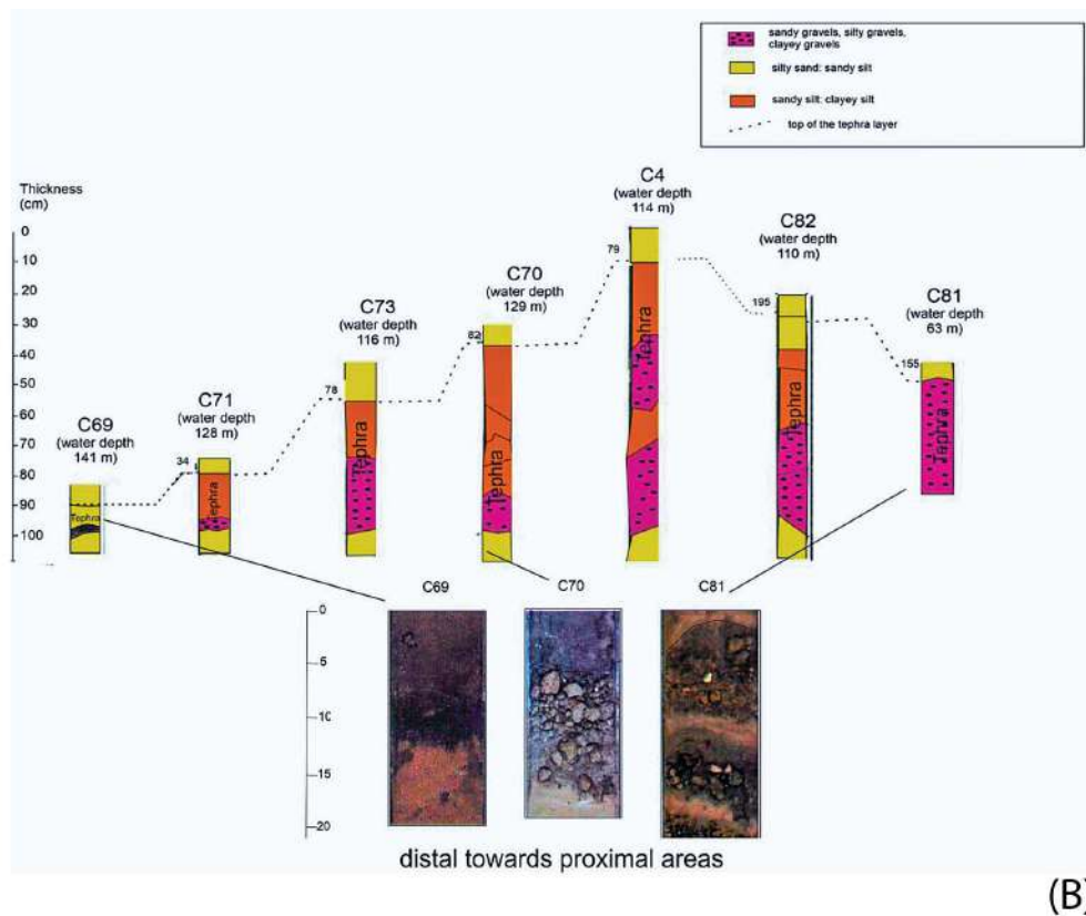
Figure 6. (A) Location map of the cores showing marine tephra in Naples Bay (modified after Aiello and Caccavale [43]). (B) Sketch stratigraphic section of the C69, C71, C73, C70, C4, C82, and C81 cores [51–53], in which the top of the tephra layer has been reported, and detailed core photographs showing the passage from distal (fine-grained) to proximal (coarse-grained) areas.
