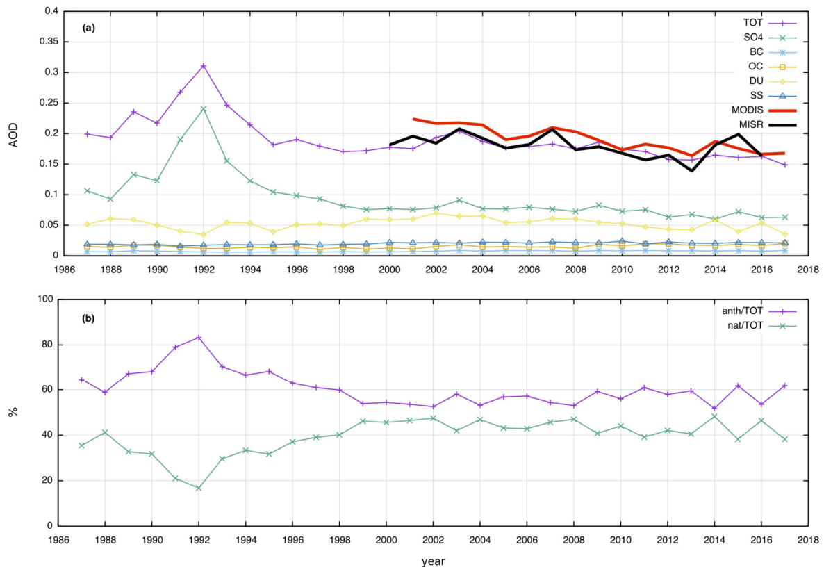
Figure 4. Time series of aerosol optical depth (AOD) for the city of Rome (a) and percentages of anthropogenic (black carbon (BC), organic carbon (OC), and \text{SO}_4 ) and natural (dust (DU), and sea salt (SS)) AOD components (b). TOT — total; nat — natural; anth — anthropogenic.
