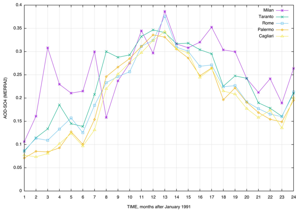
Figure 8. Time series of AOD for the SO 4 component for the five selected cities in the 1991–1992 period.
