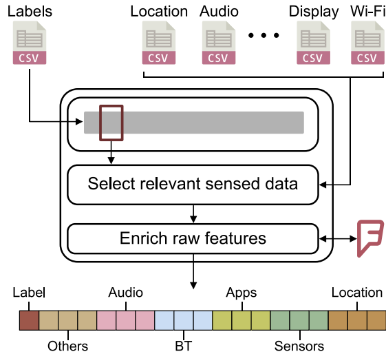
Figure 2: Dataset building process.
