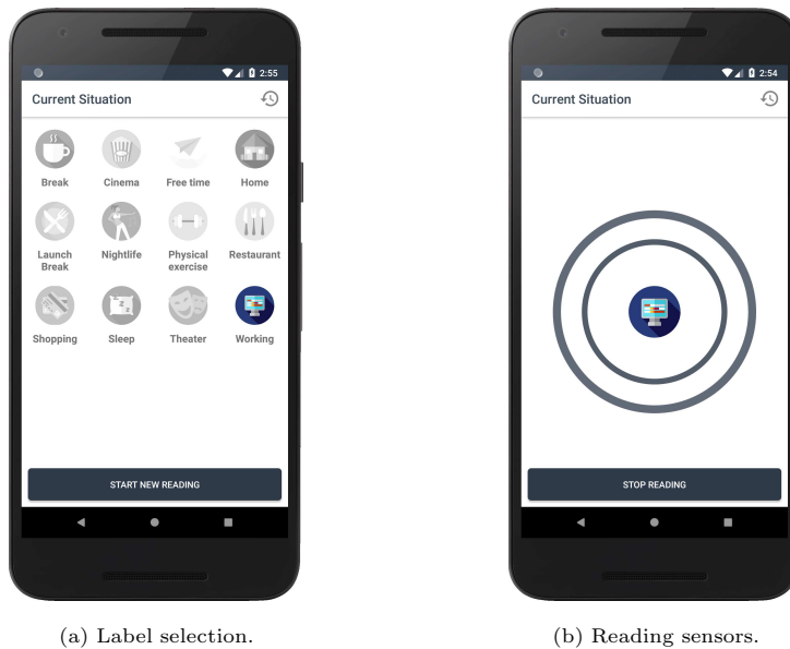
Figure 1: User Interface of the Context Labeler mobile application.
