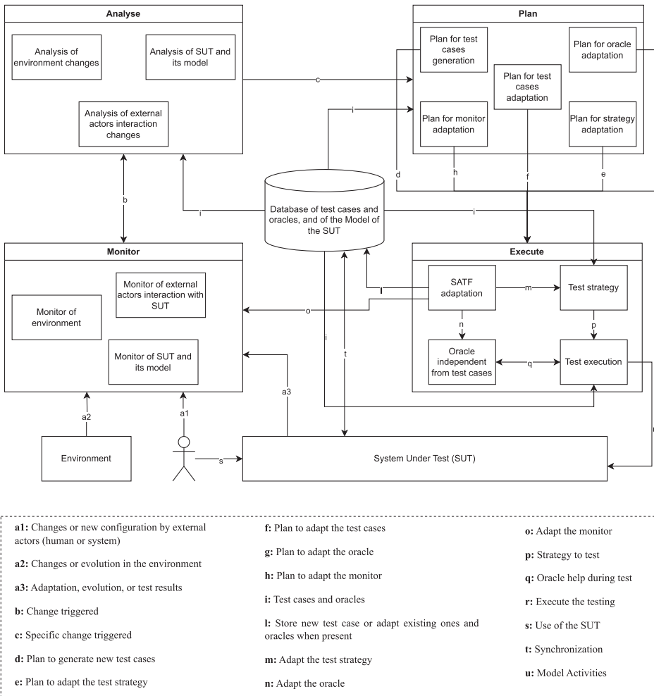
Fig. 4. Reference architecture for SATF approaches.
