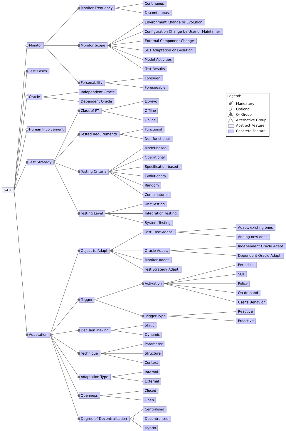
Fig. 3. Feature model of the dimensions.
