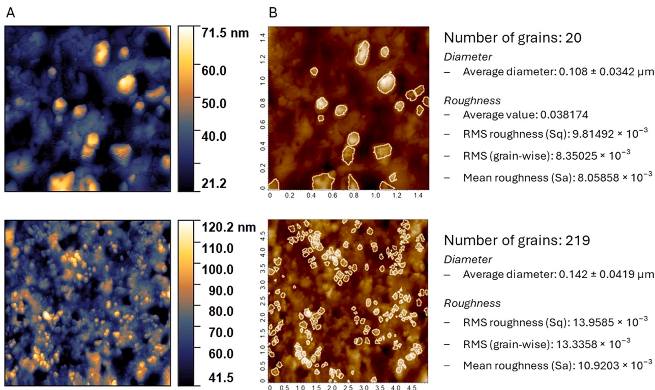
Fig. 4. Representative images of topography derived from AFM analysis of ADNVs from roasted almonds. Diameters are reported as mean value \pm standard deviation. Panel A: non-masked images; the colorimetric legend refers to the height of the object. Panel B: scanned vesicles marked as grains. RMS Sq: mean square of height irregularities (Sq); RMS (grain-wise): mean value for each grain separately; mean roughness (Sa): mean value of height irregularities.
