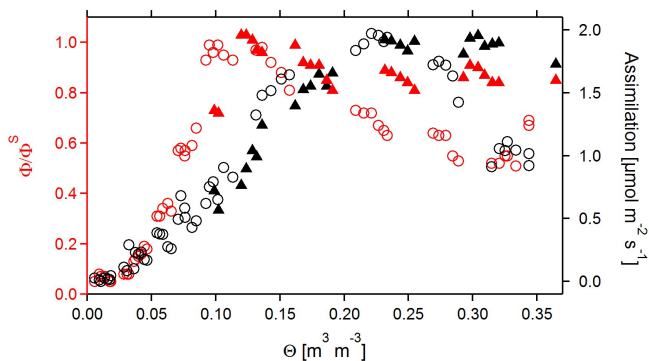
Figure 4. Normalized sabinene emissions from beech (red symbols, left scale) and rates of net photosynthesis (black symbols, right scale, multiplied by -1 ) in dependence on \Theta . Closed triangles represent data taken during a first drought period that was stopped when \Theta had fallen to 0.1 \text{ m}^3 \times \text{m}^{-3} (days 0–5 in Fig. 3), open circles represent data taken during the following period of recovery (days 6–10 in Fig. 3) until the end of the severe drought at day 17. Only data taken at a chamber temperature of 23^\circ\text{C} and a PAR of 440 \mu\text{mol m}^{-2} \text{s}^{-1} are considered.
