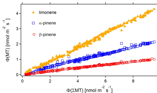
Figure 2. Correlation plot of emission rates measured for Holm oak, experiment 2. Only data measured at a PAR of 440 \mu\text{mol m}^{-2} \text{ s}^{-1} and a chamber temperature of 22^\circ\text{C} are plotted. The variation of emission rates is caused by changes in soil moisture. The high coefficients of determination ( R^2 > 0.95 ) indicate that only the strengths of the emissions was changed but not the emission pattern.
