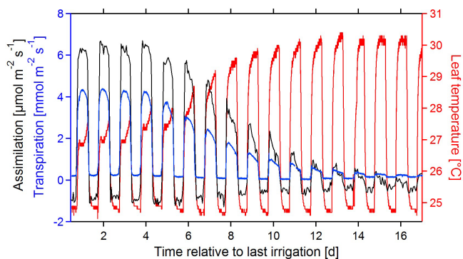
Figure 1. Temporal development of transpiration (blue trace, left hand y axis) and leaf temperature (red trace, right hand y axis, average of three leaves) at the example of Holm oak, experiment 1. The plant was irrigated at day 0 ( \Theta = 0.4 \text{ m}^3 \times \text{m}^{-3} ). At the end of the drought period \Theta had fallen to 0.05 \text{ m}^3 \times \text{m}^{-3} . Chamber temperature 25^\circ\text{C} , \text{PAR} = 600 \mu\text{mol m}^{-2} \text{ s}^{-1} .
