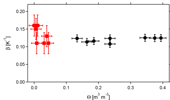
Figure 6. Temperature coefficient \beta for \alpha -pinene emissions from Holm oak (experiment 3) at different soil moisture. Black circles represent the data obtained without impacts of drought on MT emissions. Red squares represent the data obtained for \Theta < 0.06 \text{ m}^3 \times \text{m}^{-3} after correcting for the drought-induced decrease of emissions. Errors in \beta were about \pm 0.01 \text{ K}^{-1} for the data obtained without drought stress. For the data obtained during drought stress the errors from the normalization procedure had to be taken into account and errors in \beta are estimated to be \pm 0.03 \text{ K}^{-1} . Error in \Theta is estimated to be \pm 0.016 \text{ m}^3 \times \text{m}^{-3} .
