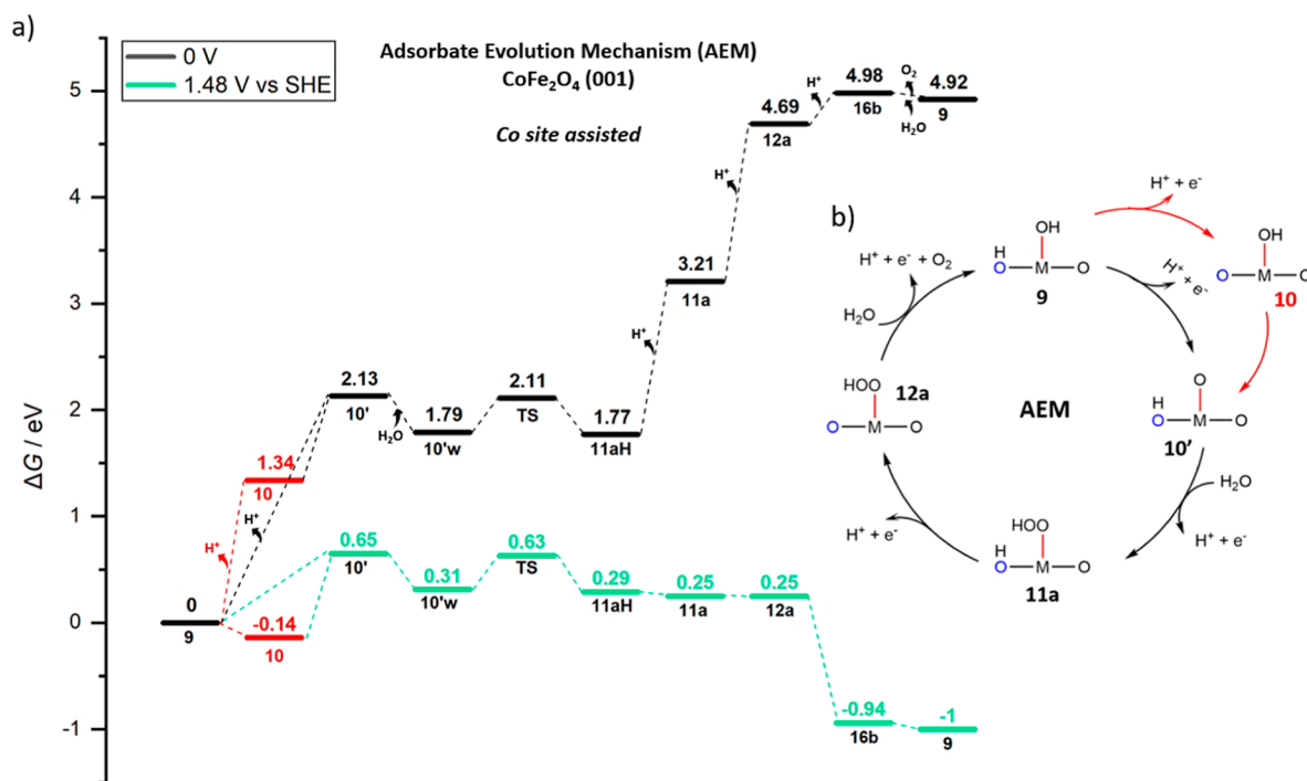
Figure 9. (a) Free energy ( G , eV) profiles that represent AEM assisted by Co sites catalytic cycle of OER on (001) CoFe_2O_4 at U = 0 V (black) and U = 1.48 V (green). (b) overarching mechanistic catalytic cycle labeled with the same notations on the intermediates used in the free energy profile and Figure 7.
