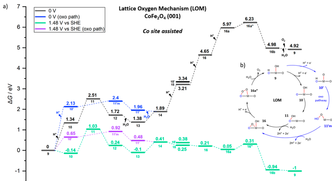
Figure 8. (a) Free energy ( G , eV) profiles that represent for the LOM assisted by Co sites, OER intermediates (shown in Figure 7) of catalytic cycle on (001) CoFe_2O_4 at U = 0 V (black, blue for the oxo path) and U = 1.48 V vs SHE (green and purple for the oxo path). (b) Overarching mechanistic catalytic cycle labeled with the same notations on the intermediates used in the free energy profile and Figure 7.
