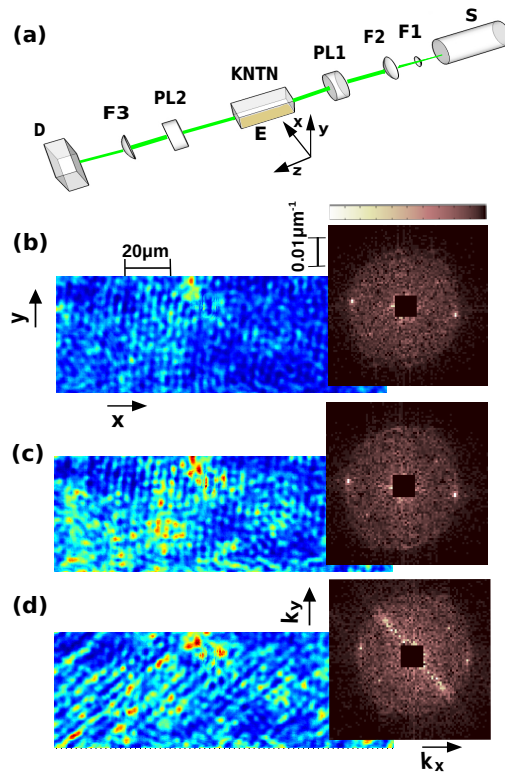
Fig. 2. (a) Cross-polarizer setup and (b) transmission microscopy images (intensity is in arbitrary units) in zero-field-cooling at T = 287\text{K} and (c) at T = T_m = 285.5\text{K} ; (d) applying a 0.85\text{kV/cm} dc field the glassy state at T_m turns into ferroelectric domains with geometrically fixed boundaries at 45^\circ with respect to the principal axes of the crystal. Normalized intensity Fourier transform (insets in (b), (c) and (d)) that highlights the appearance of a diagonal feature in the spectrum associated to ferroelectric domains. The added spectrum in (d) is continuous, with no fixed periodicity, typical of a globally disordered state.
