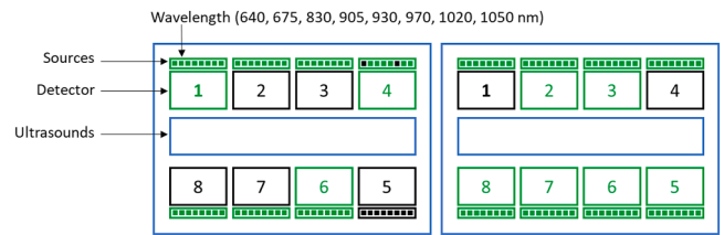
Fig. 2. Schematic representation of the SOLUS probe (shown in Fig. 1, right). In each optode, the big window represents the detector, the small window represents the array of sources and each single filled square a single source at a certain wavelength. The schematic is used to depict the current status of the first (left) and second (right) SOLUS probes: green color highlights active optical elements.
