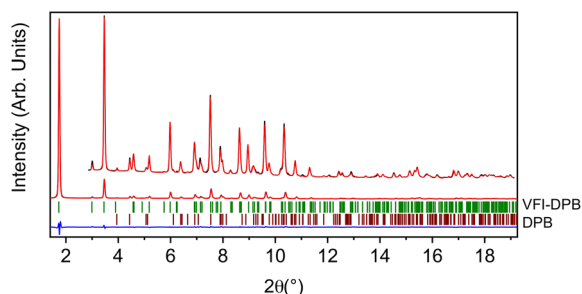
Fig. 2 Experimental (black), calculated (red) and difference (blue) profiles ( \lambda = 0.4957 \text{ \AA} ) for the Rietveld refinement of the DPB-filled VFI (VFI-DPB) and DPB mixture. Vertical bars indicate the calculated positions of the Bragg reflections of VFI-DPB (above) and DPB (below). A vertical zoom of the patterns from 3–19.2° is given in the inset.
