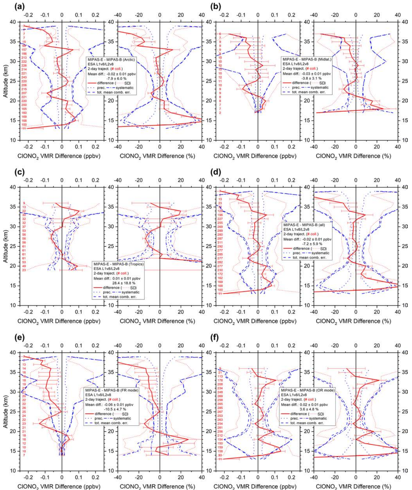
Figure 10. Same as Fig. 3 but for CION 2 .
