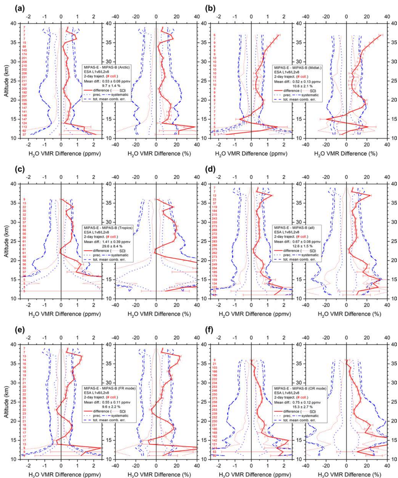
Figure 3. Mean absolute and relative H 2 O VMR differences of all trajectory match collocations (red numbers) between MIPAS-E and MIPAS-B (red solid line), including standard deviation (red dotted lines) and standard error of the mean (plotted as error bars). Precision (blue dotted lines), systematic (blue dash-dotted lines), and total (blue dashed lines) mean combined errors are shown too. Arctic (a), midlatitude (b), tropics (c), all FR plus OR (d), FR mode (e), and OR mode (f) collocations. For details, see text.
