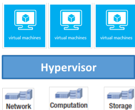
Figure 10 Virtual Machines
