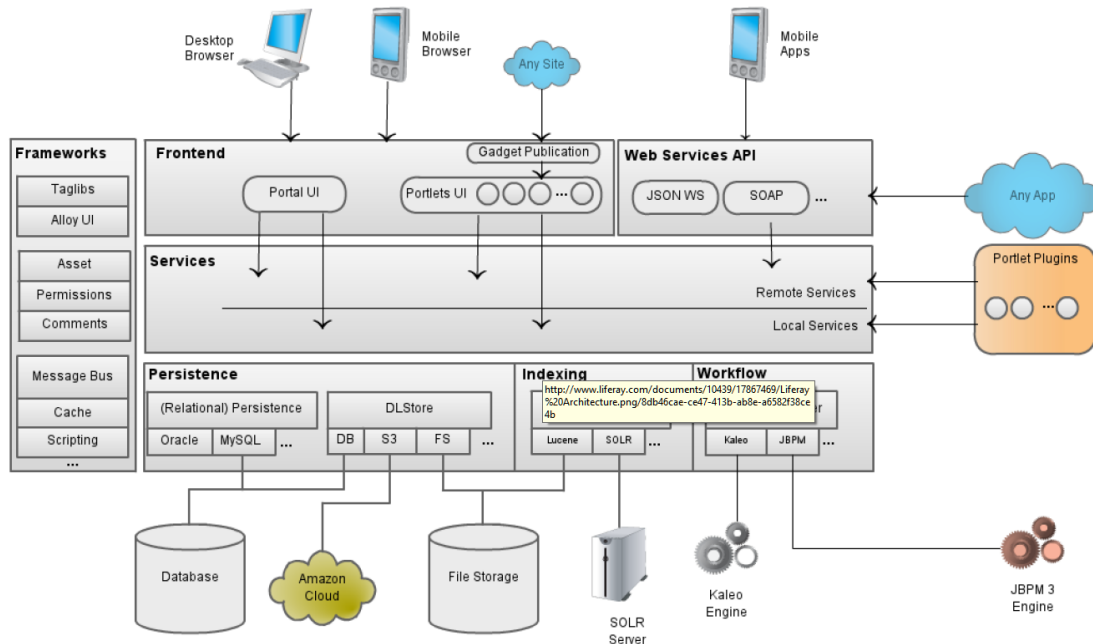
Figure 45 Liferay architecture
