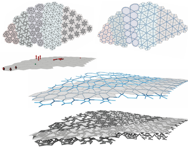
Fig. 12. Example A results: pattern tiling and the corresponding reduced model on top; simulation setup; reduced model deformed shape (blue) and ground-truth deformed shape (gray).
