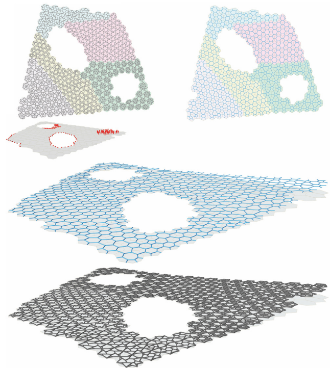
Fig. 13. Example B results: pattern tiling and the corresponding reduced model on top; simulation setup; reduced model deformed shape (blue) and ground-truth deformed shape (gray).
