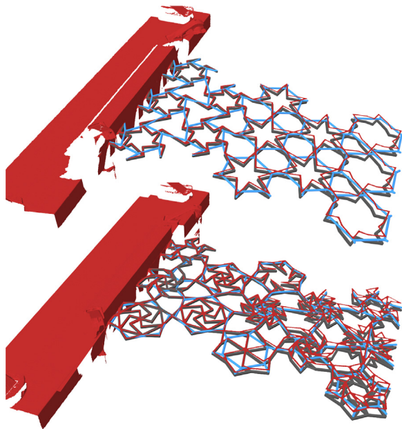
Fig. 15. Physical tests (red) in comparison with deformations of the pattern (dark gray) and the reduced model (blue).
