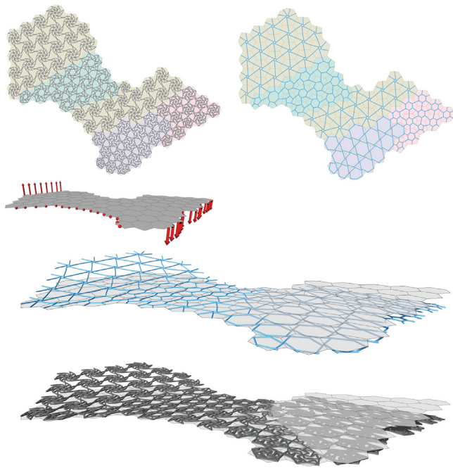
Fig. 14. Example C results: pattern tiling and the corresponding reduced model on top; simulation setup; reduced model deformed shape (blue) and ground-truth deformed shape (gray).
