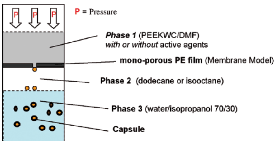
Fig. 2 - Scheme of capsule formation unit.
