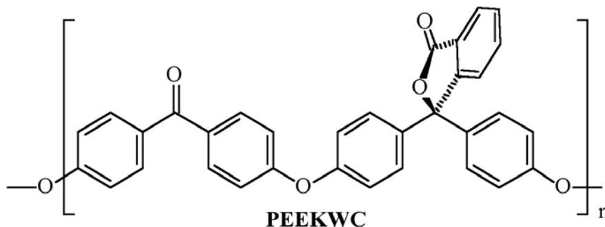
Fig. 1 - Chemical structure of PEEKWC.
