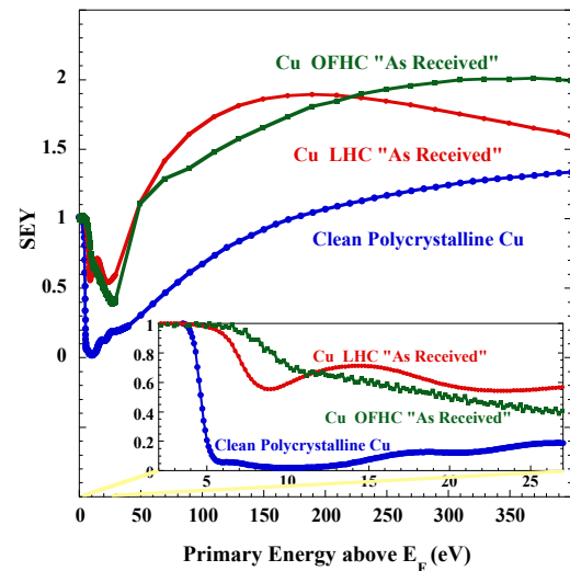
Figure 1: Experimental SEY curves of an OFHC "as received" Cu; a LHC "as received" Cu and of a clean polycrystalline Cu in the energy region between 0 and 400 eV above E_F . In the inset we zoom on the LE-SEY region between 2 and 27 eV above E_F .
