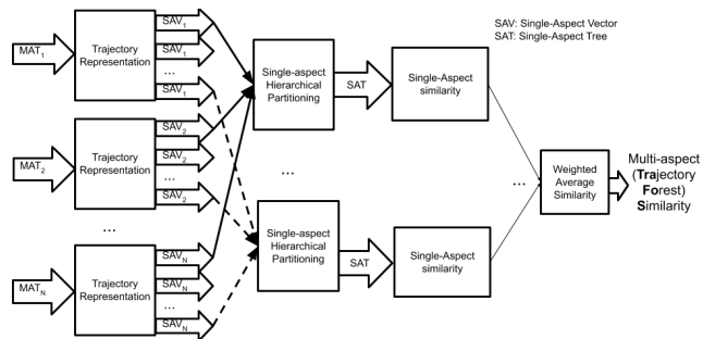
Figure 2: The steps of TraFoS similarity for MATs.
