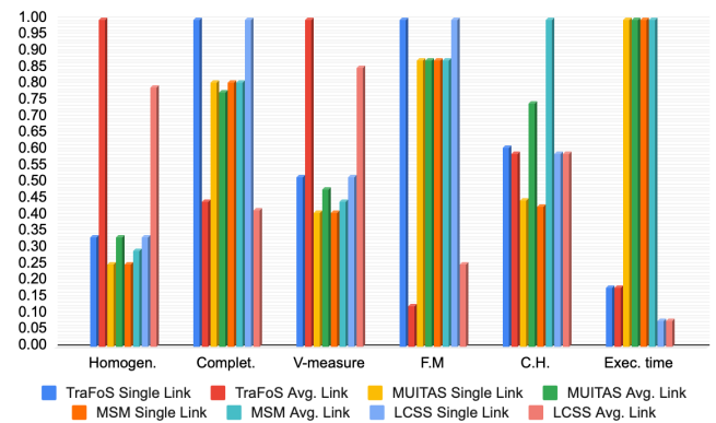
Figure 5: Summarizing evaluation results and execution time.
