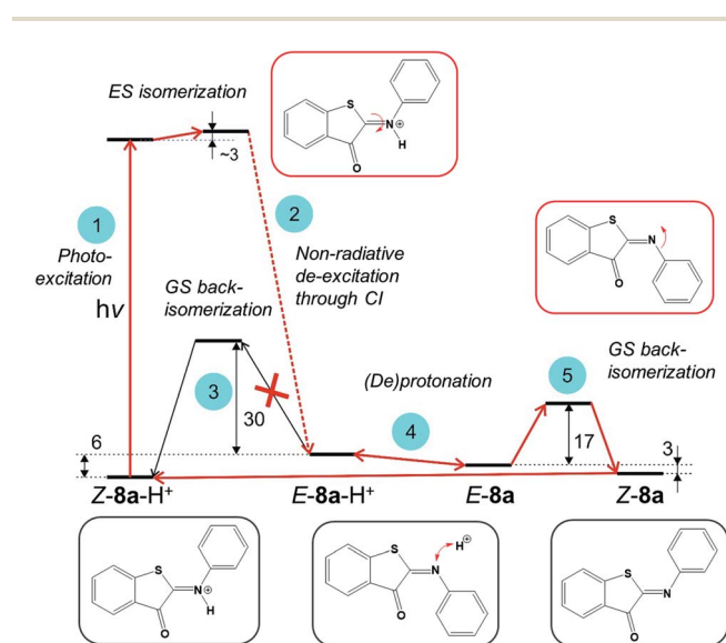
Fig. 6 Reaction mechanism of photoisomerization of ITIs in an acidic environment as revealed by theoretical investigations. The GS energy values (in kcal mol -1 ) reported here for compound 8a in DCM were obtained employing the composite DLPNO-CCSD(T)/M06-2X/SMD approach. See the text for computational details and discussion of individual steps.
