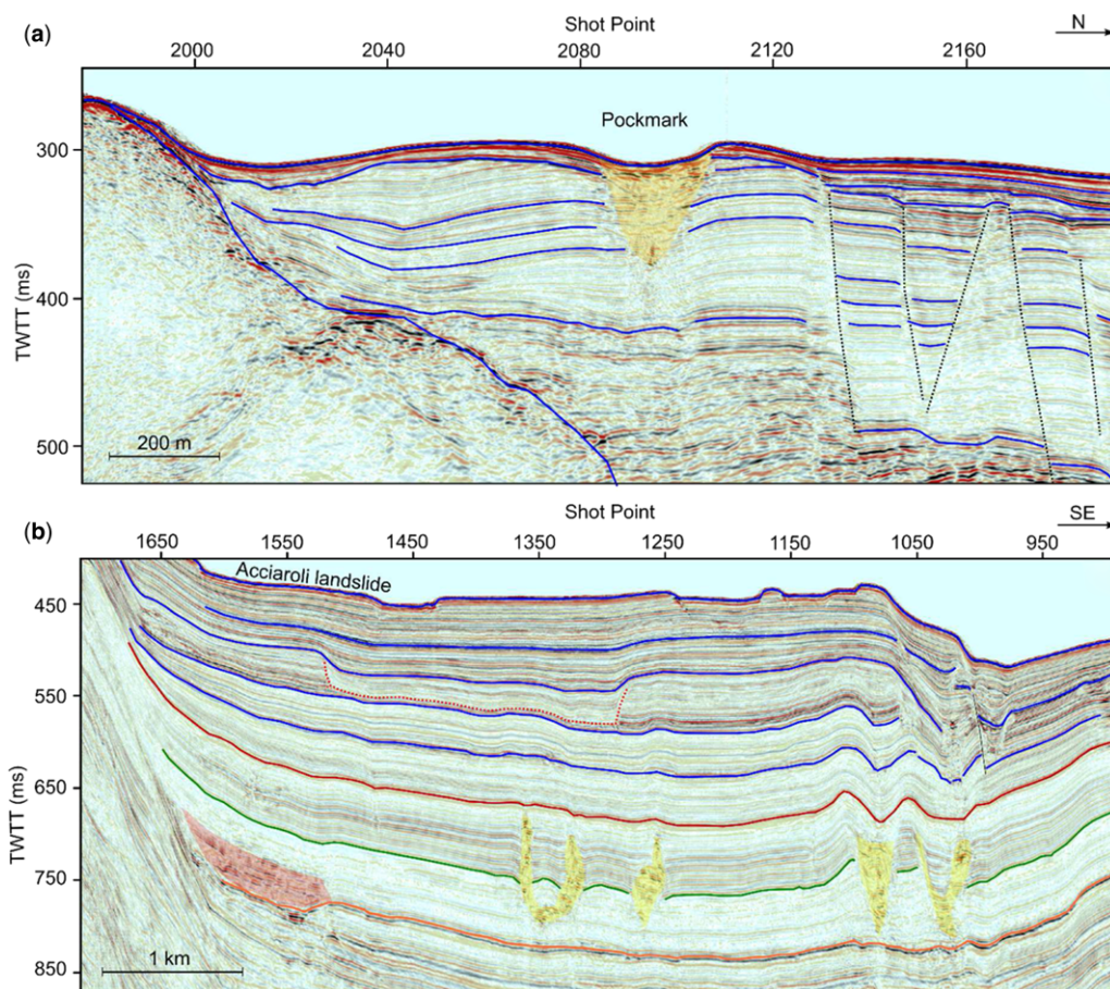
Fig. 6. More evidence of fluid escape appears within 15 km SE of the landslide, along multichannel seismic profile LIC_05 and LIC_6. (a) The presence of a surficial pockmark indicates recent fluid-escape activity. The pockmark is visible both on the seismic data (multichannel seismic profile LIC_05) and the bathymetric grid. Vertical exaggeration is \times 3.8 . (b) The image (multichannel seismic profile LIC_06) shows in yellow the presence of anomalous high-amplitude and concave-upwards signals, which affect the same layer interval hosting the buried pockmark (Fig. 5). A buried landslide scar is identified, with a dashed line, at a depth of approximately 40 m. An additional landslide deposit, at a depth of approximately 250 m, is highlighted in red. Vertical exaggeration is \times 9 . The location of both seismic profiles is shown in Figure 1b.
